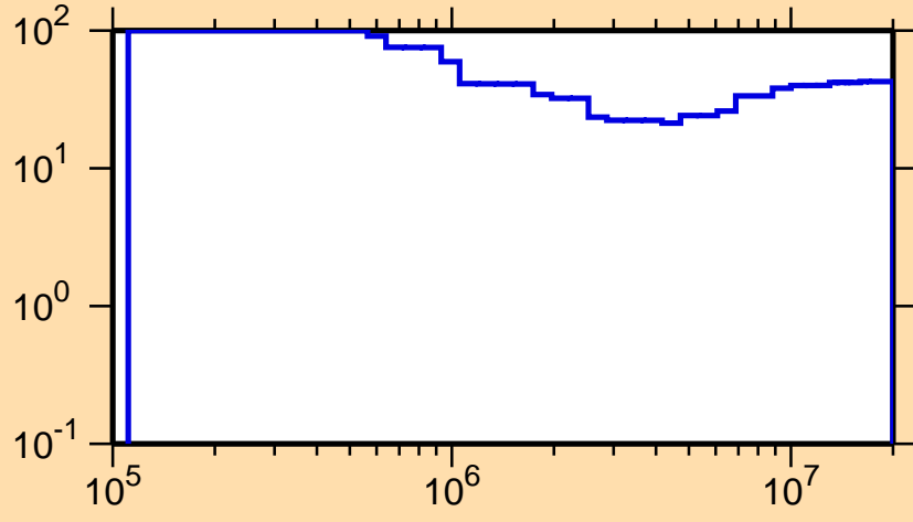
\Delta\sigma/\sigma vs. E for ^{126}\text{La}(n,n\text{cont.})
