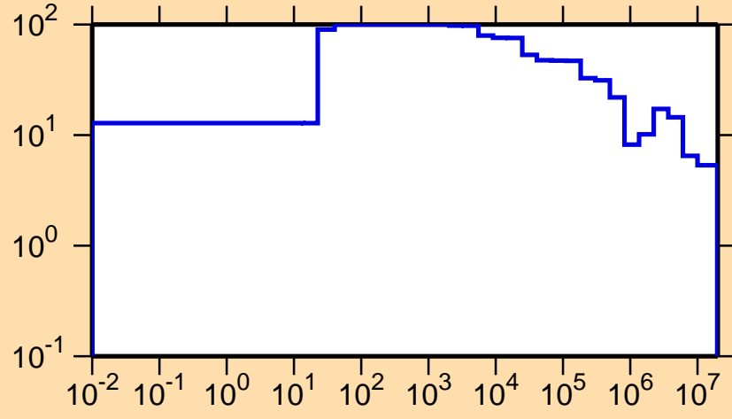
\Delta\sigma/\sigma vs. E for ^{126}\text{La}(n,el.)
