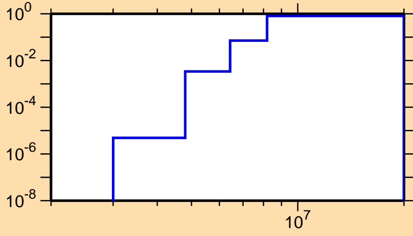
\sigma vs. E for ^{126}\text{La}(n,np)
