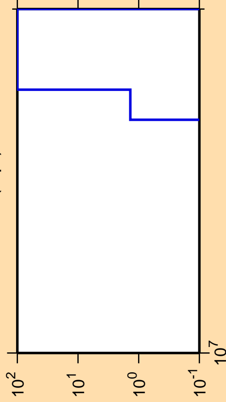
\Delta\sigma/\sigma vs. E for ^{127}\text{La}(n,pt)
