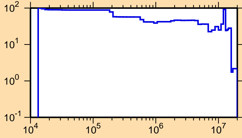
\Delta\sigma/\sigma vs. E for ^{127}\text{La}(n,n_1)
