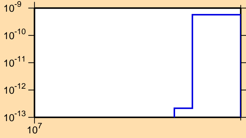
\sigma vs. E for ^{127}\text{La}(n,pt)
