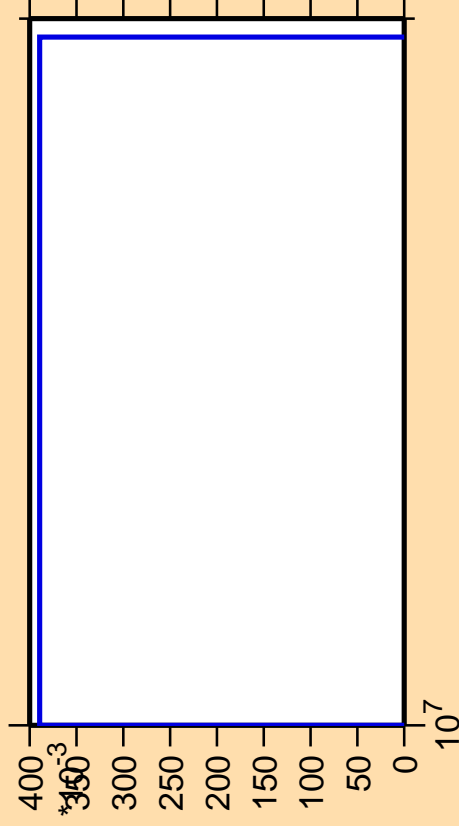
\Delta\sigma/\sigma vs. E for ^{127}\text{La} (mt 34)
