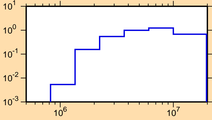
\sigma vs. E for ^{127}\text{La}(n,n\text{cont.})
