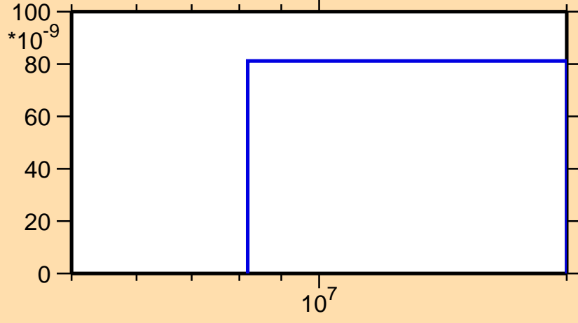
\sigma vs. E for ^{127}\text{La}(n,\text{pd})
