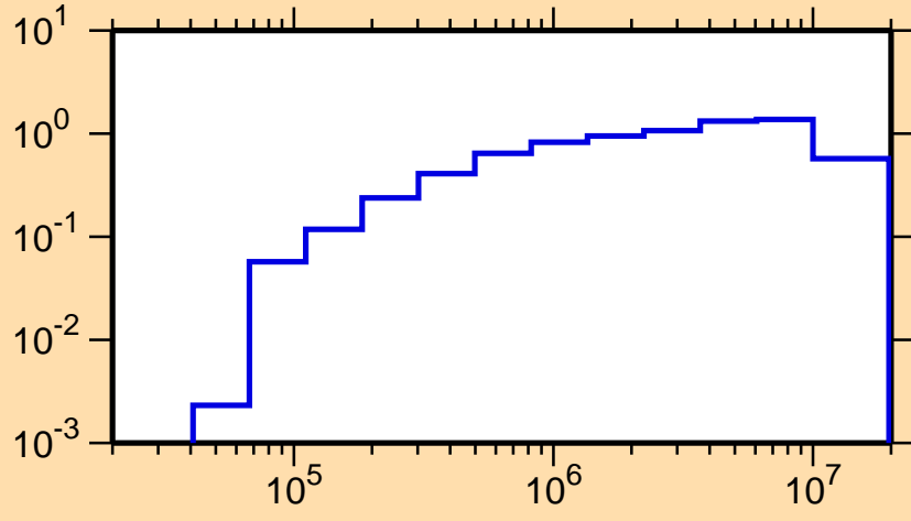
\sigma vs. E for ^{127}\text{La}(n,\text{inel.})
