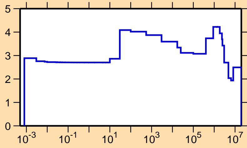
\sigma vs. E for ^{127}\text{La}(n,\text{el.})
