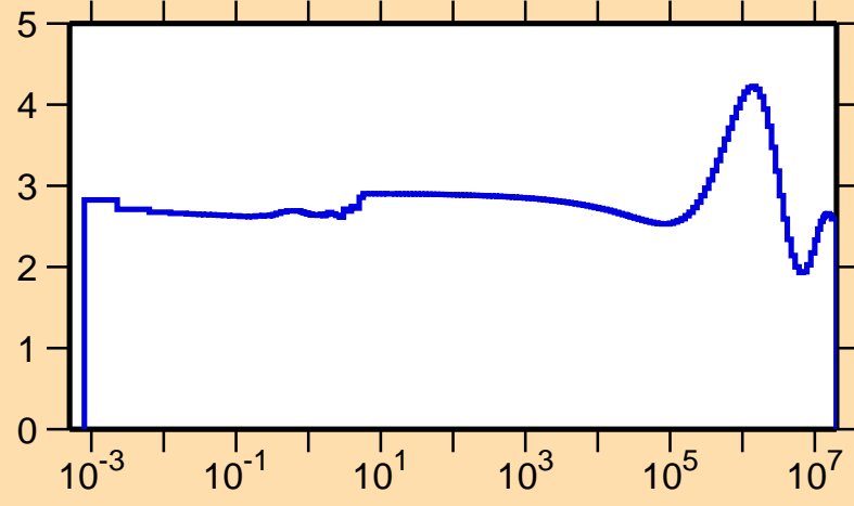
\sigma vs. E for ^{128}\text{La}(n,\text{el.})
