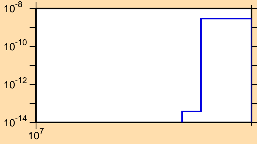
\sigma vs. E for ^{128}\text{La}(n,nt)
