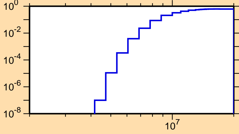
\sigma vs. E for ^{128}\text{La}(n,np)
