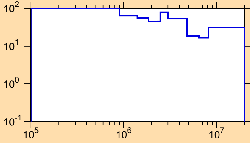
\Delta\sigma/\sigma vs. E for ^{128}\text{La}(n,n\text{cont.})
