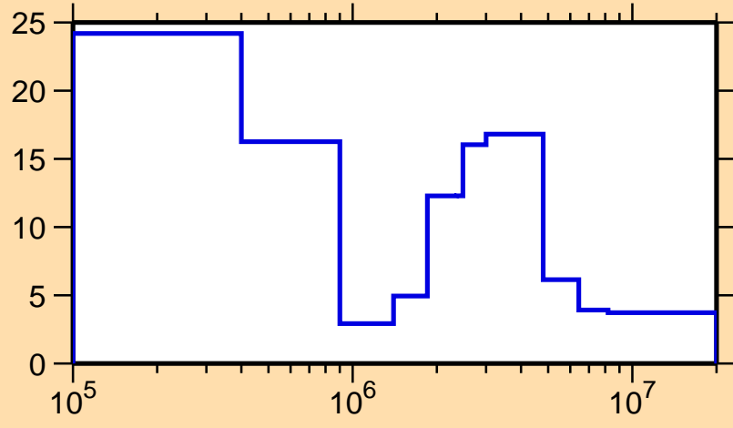
\Delta\sigma/\sigma vs. E for ^{128}\text{La}(n,el.)
