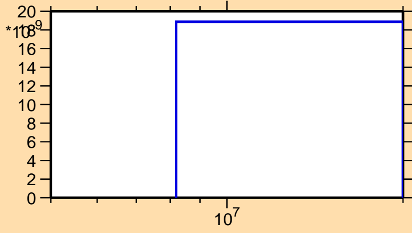
\sigma vs. E for ^{128}\text{La} (mt 45)
