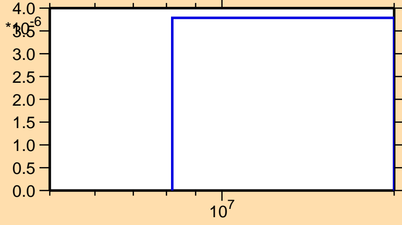
\sigma vs. E for ^{128}\text{La}(n,\text{nd})
