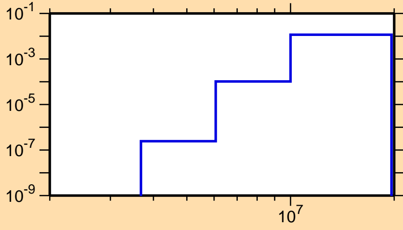
\sigma vs. E for ^{128}\text{La}(n,d)
