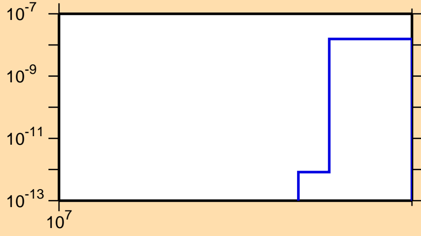
\sigma vs. E for ^{129}\text{La}(n,nt)
