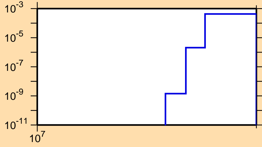
\sigma vs. E for ^{129}\text{La}(n,2np)
