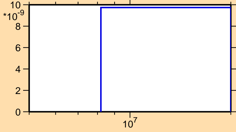
\sigma vs. E for ^{129}\text{La} (mt 45)
