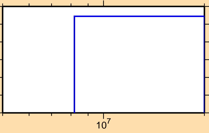
\sigma vs. E for ^{129}\text{La} (mt 34)
