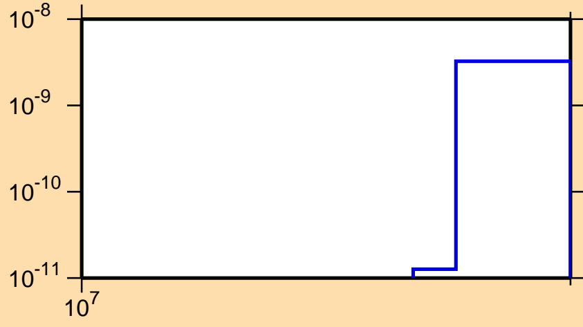
\sigma vs. E for ^{130}\text{La}(n,\text{pt})
