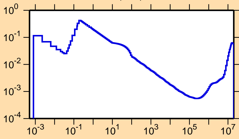
\sigma vs. E for ^{130}\text{La}(n,\alpha)
