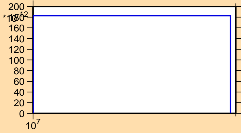
\sigma vs. E for ^{130}\text{La}(n,pd)
