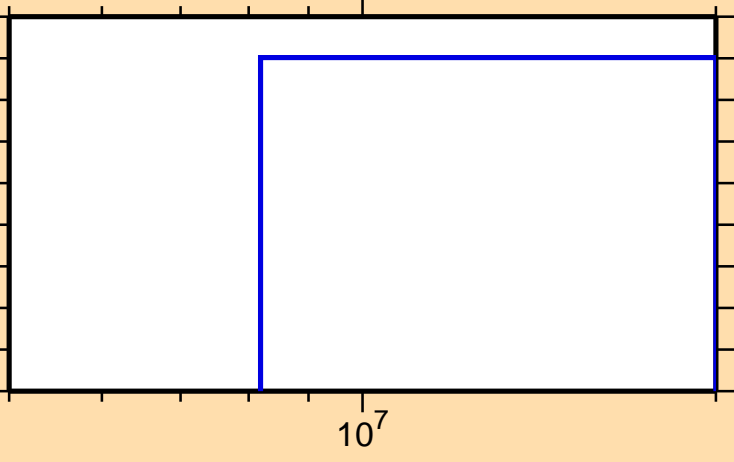
\sigma vs. E for ^{130}\text{La}(n,pd)
