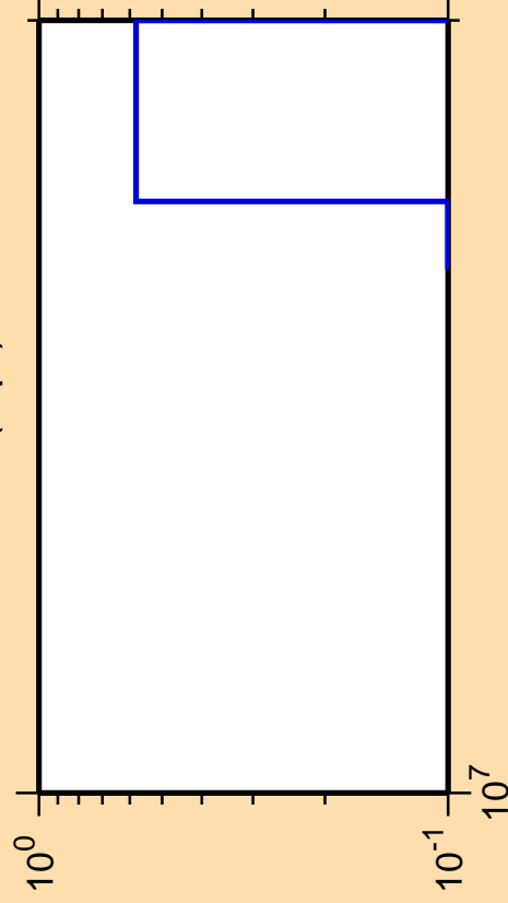
\Delta\sigma/\sigma vs. E for ^{131}\text{La}(n,\text{pt})
