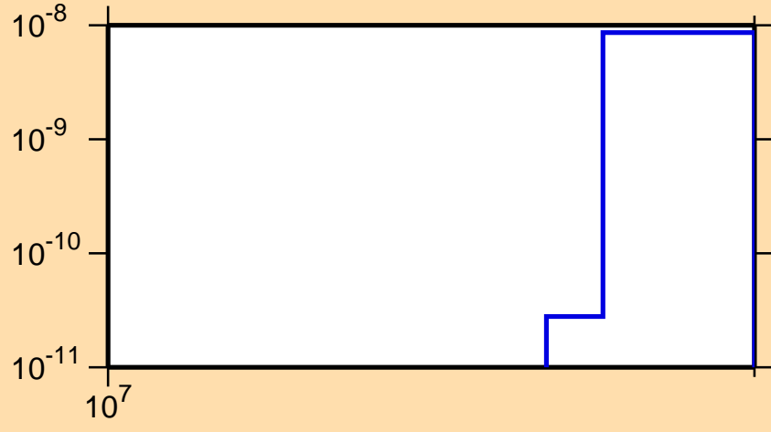
\sigma vs. E for ^{131}\text{La}(n,2n\alpha)
