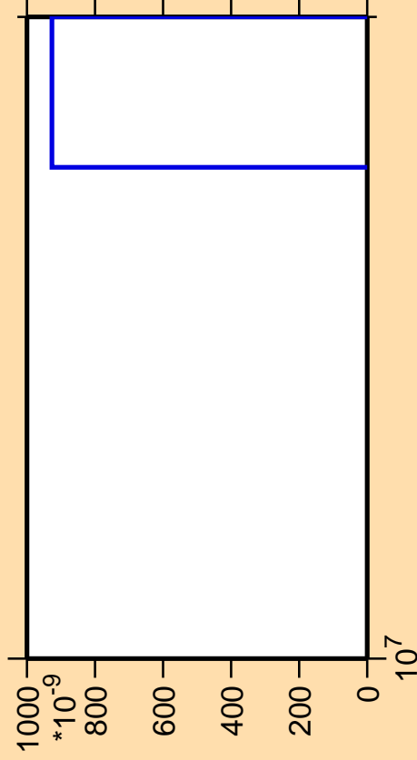
\Delta\sigma/\sigma vs. E for ^{131}\text{La} (mt 11)
