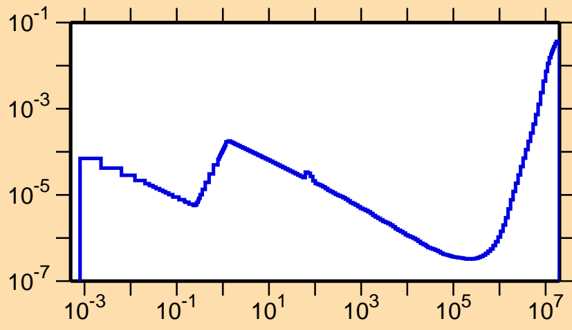
\sigma vs. E for ^{131}\text{La}(n,\alpha)
