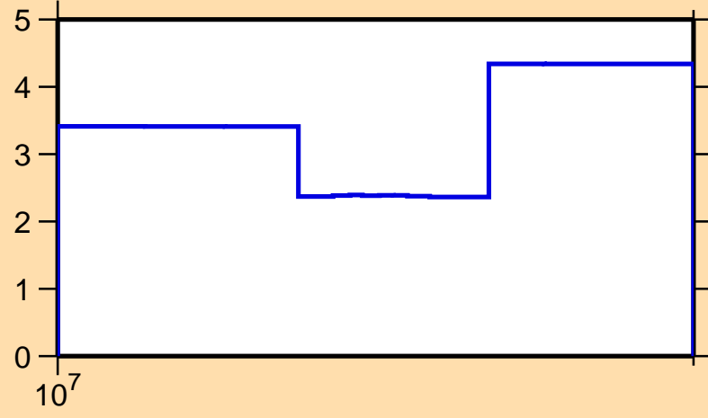
\Delta\sigma/\sigma vs. E for ^{131}\text{La}(n,\text{el.})
