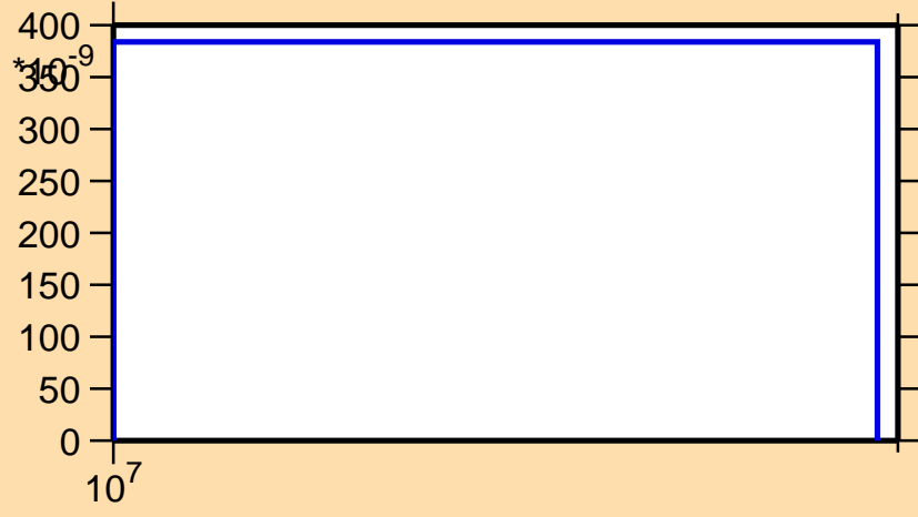
\sigma vs. E for ^{131}\text{La}(n,3n)
