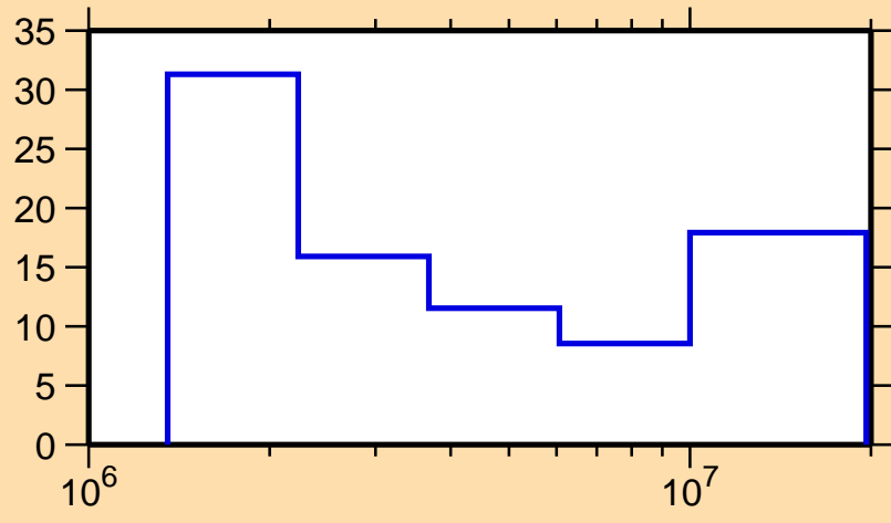
\Delta\sigma/\sigma vs. E for ^{131}\text{La}(n,n\text{cont.})
