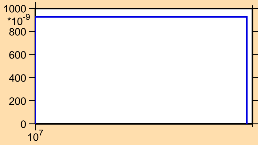
\sigma vs. E for ^{131}\text{La}(n,2np)
