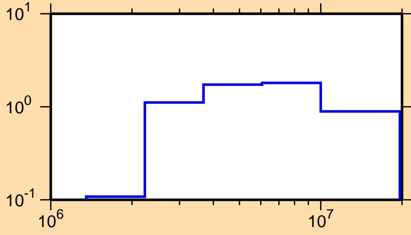
\sigma vs. E for ^{131}\text{La}(n,n\text{cont.})
