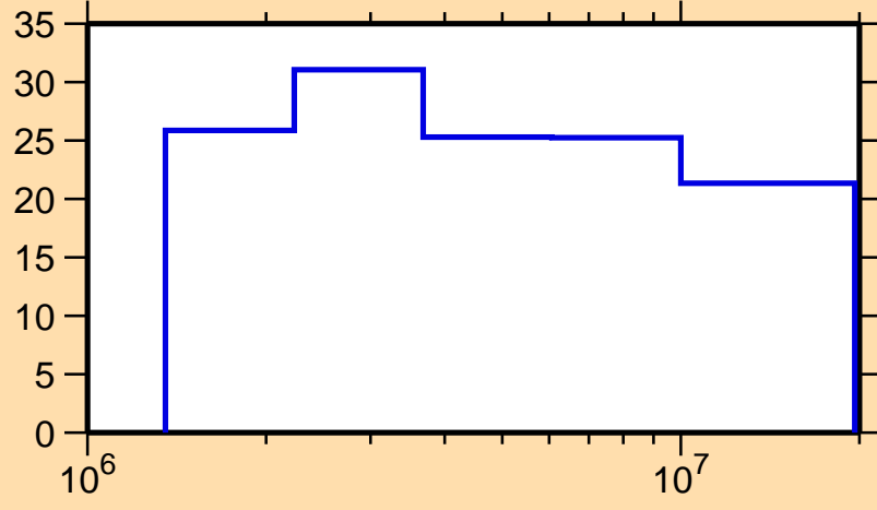
\Delta\sigma/\sigma vs. E for ^{131}\text{La}(n,n_1)
