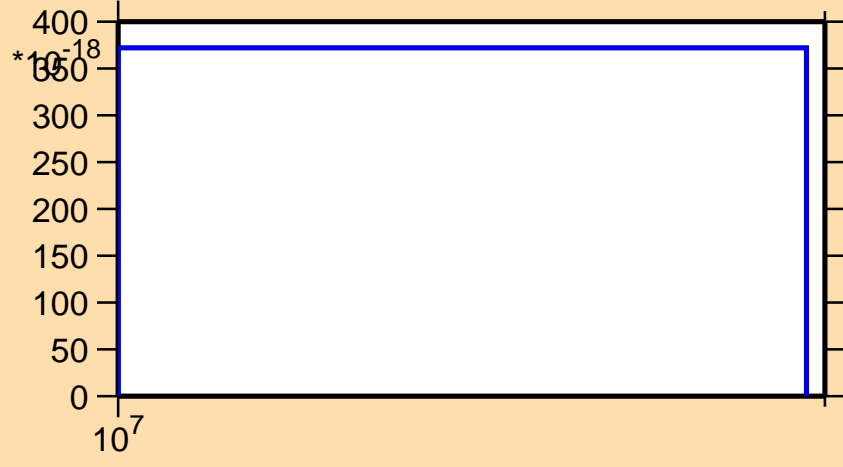
\sigma vs. E for ^{131}\text{La}(n,\text{pt})
