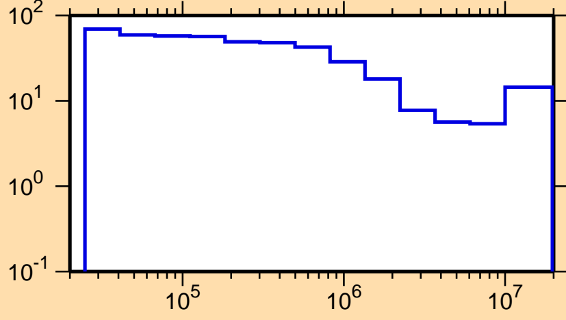
\Delta\sigma/\sigma vs. E for ^{131}\text{La}(n,\text{inel.})
