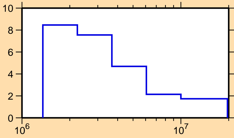
\Delta\sigma/\sigma vs. E for ^{131}\text{La}(n,\text{tot.})
