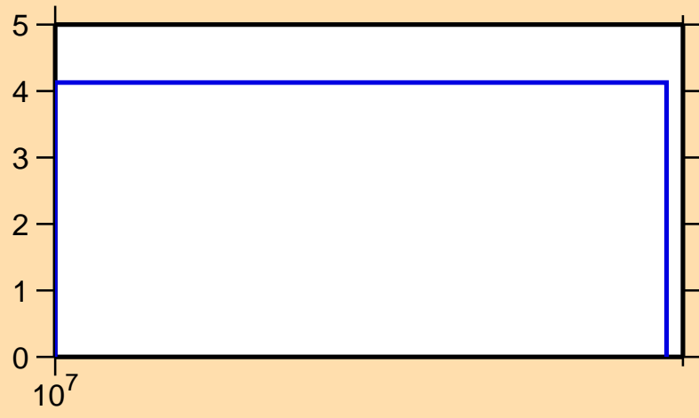
\Delta\sigma/\sigma vs. E for ^{131}\text{La}(n,\text{nonel.})
