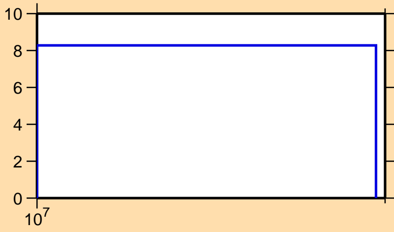
\Delta\sigma/\sigma vs. E for ^{131}\text{La}(n,2n)
