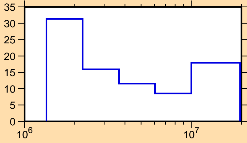
\Delta\sigma/\sigma vs. E for ^{131}\text{La}(n,n\text{cont.})
