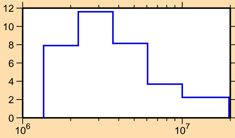
\Delta\sigma/\sigma vs. E for ^{131}\text{La}(n,\text{el.})
