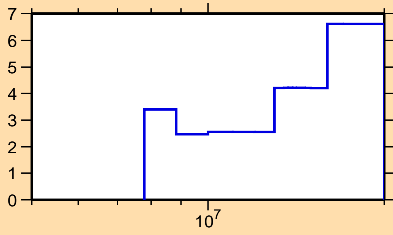
\Delta\sigma/\sigma vs. E for ^{132}\text{La}(n,\text{el.})
