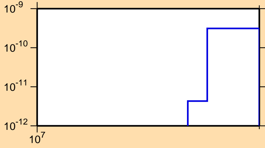
\sigma vs. E for ^{132}\text{La}(n,pd)
