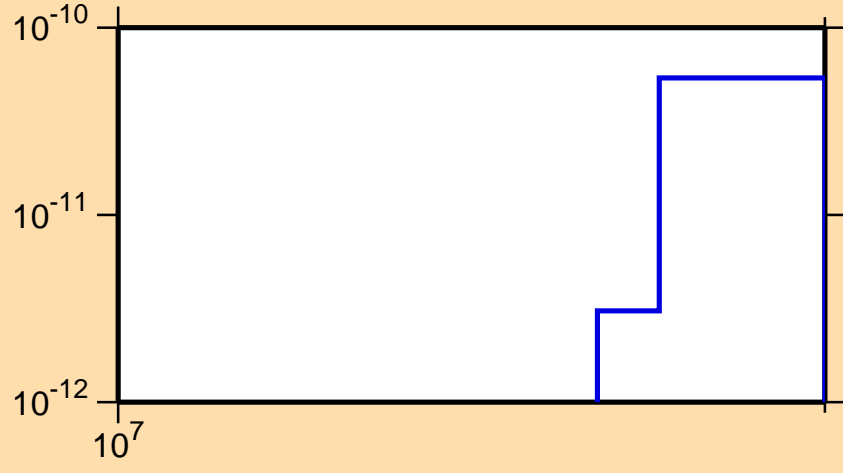
\sigma vs. E for ^{132}\text{La}(\text{mt117})
