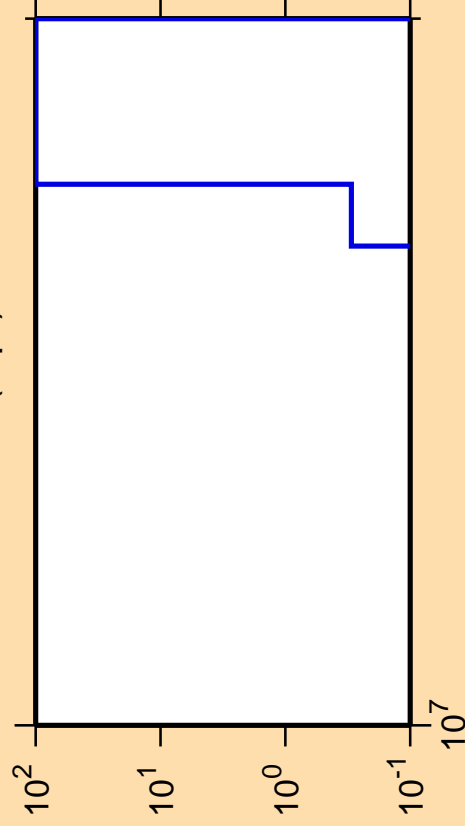
\Delta\sigma/\sigma vs. E for ^{132}\text{La}(n,\text{pt})
