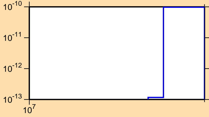
\sigma vs. E for ^{132}\text{La}(n,\text{pt})
