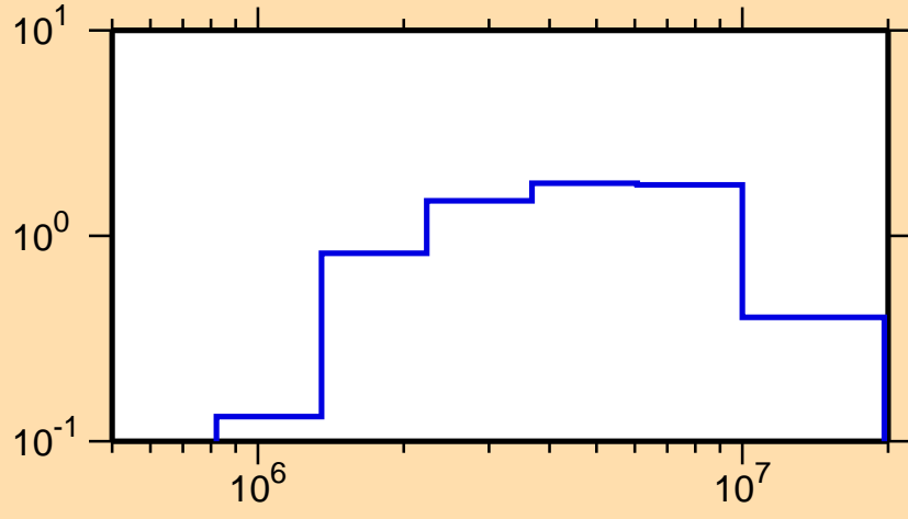
\sigma vs. E for ^{132}\text{La}(n,n\text{cont.})
