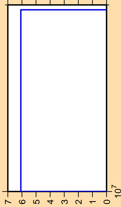
\Delta\sigma/\sigma vs. E for ^{132}\text{La} (mt 45)
