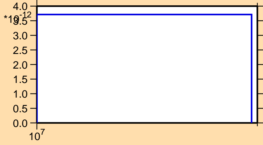
\sigma vs. E for ^{132}\text{La}(n,\text{pd})
