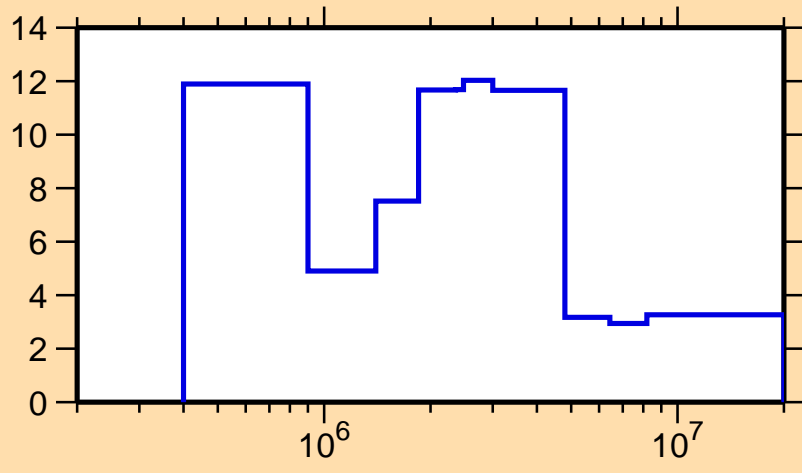
\Delta\sigma/\sigma vs. E for ^{132}\text{La}(n, el.)
