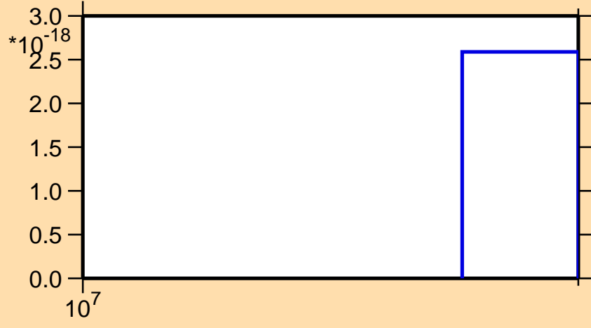
\sigma vs. E for ^{133}\text{La} (mt 11)
