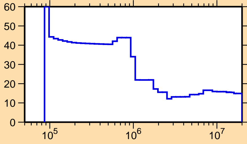
\Delta\sigma/\sigma vs. E for ^{133}\text{La}(n,n_1)
