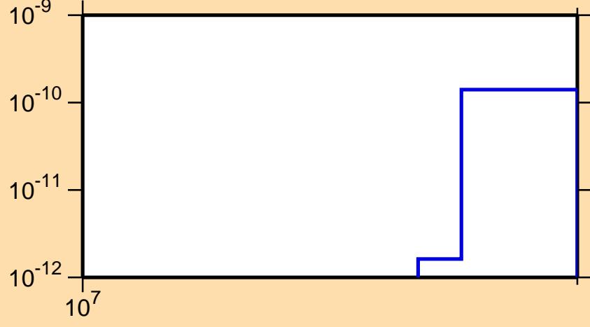
\sigma vs. E for ^{133}\text{La}(n,pd)
