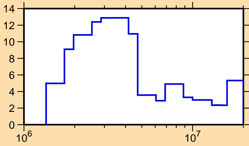
\Delta\sigma/\sigma vs. E for ^{133}\text{La}(n,\text{el.})
