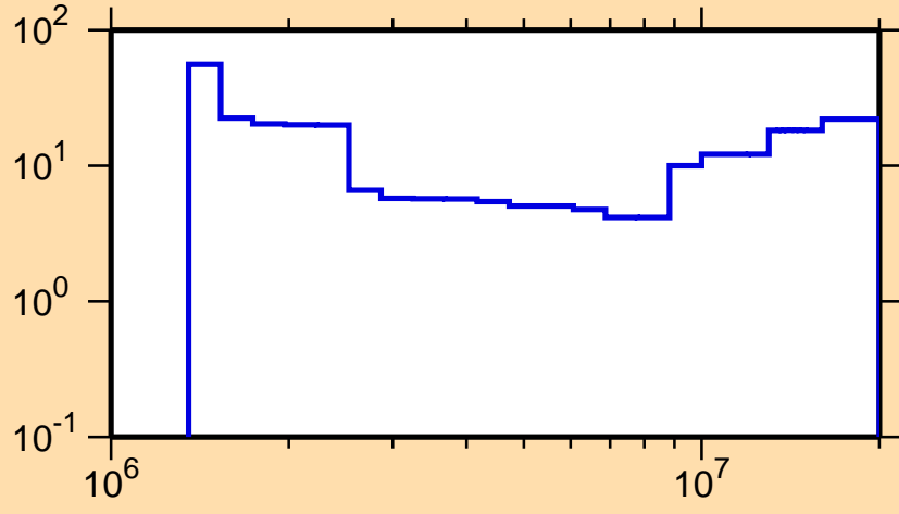
\Delta\sigma/\sigma vs. E for ^{133}\text{La}(n,n\text{cont.})
