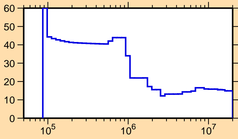
\Delta\sigma/\sigma vs. E for ^{133}\text{La}(n,n_1)
