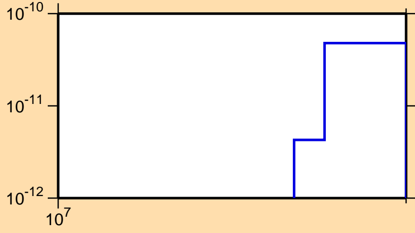
\sigma vs. E for ^{133}\text{La}(\text{mt117})
