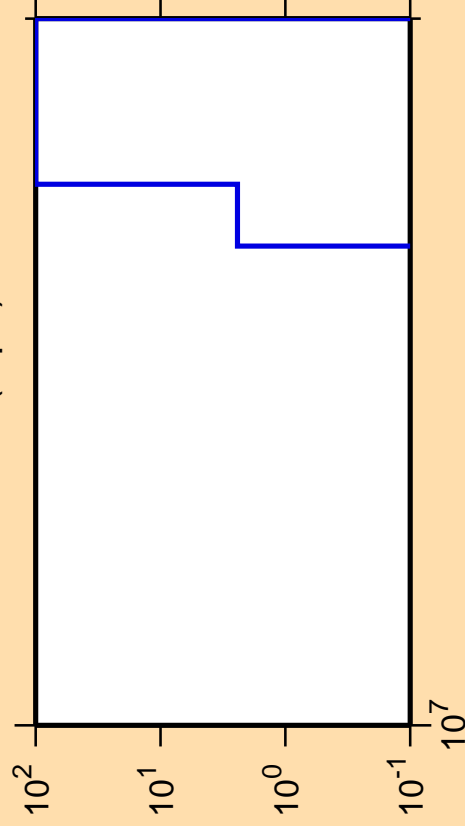
\Delta\sigma/\sigma vs. E for ^{133}\text{La}(n,pd)
