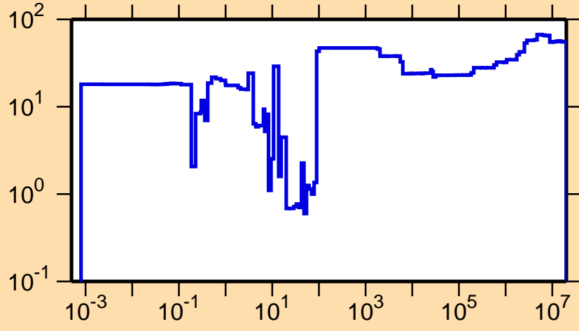
\Delta\sigma/\sigma vs. E for ^{133}\text{La}(n,\gamma)
