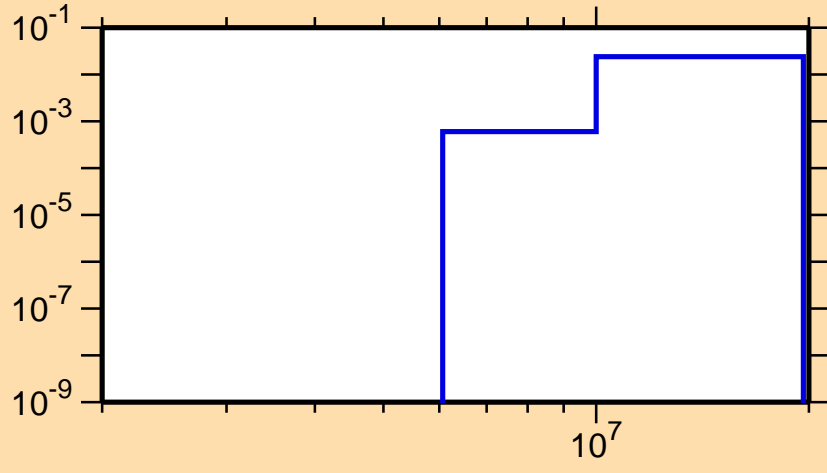
\sigma vs. E for ^{133}\text{La}(n,np)
