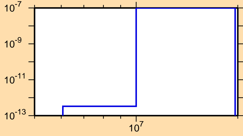
\sigma vs. E for ^{133}\text{La}(n,p\alpha)
