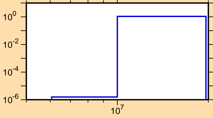
\sigma vs. E for ^{133}\text{La}(n,2n)
