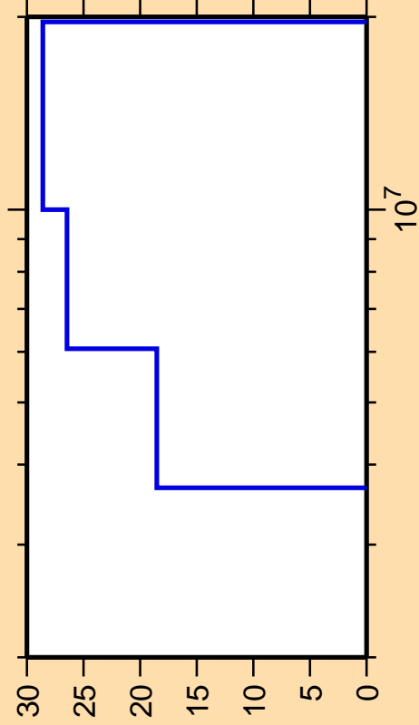
\Delta\sigma/\sigma vs. E for ^{133}\text{La}(n,np)
