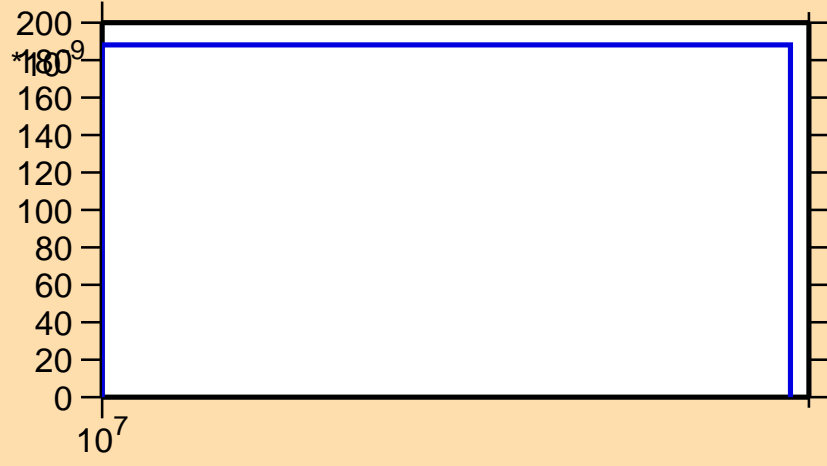
\sigma vs. E for ^{133}\text{La}(n,2np)
