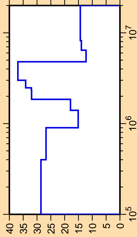
\Delta\sigma/\sigma vs. E for ^{133}\text{La}(n,n_3)
