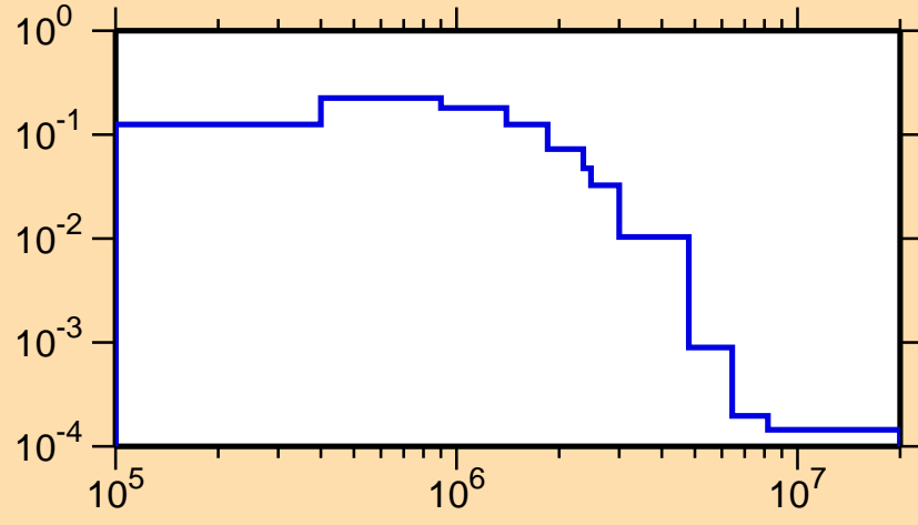
\sigma vs. E for ^{133}\text{La}(n,n_3)
