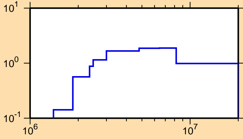
\sigma vs. E for ^{133}\text{La}(n,n\text{cont.})
