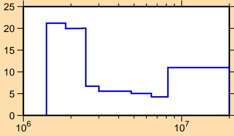
\Delta\sigma/\sigma vs. E for ^{133}\text{La}(n,n\text{cont.})
