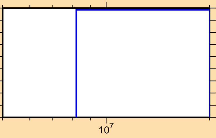
\sigma vs. E for ^{133}\text{La}(n,2np)
