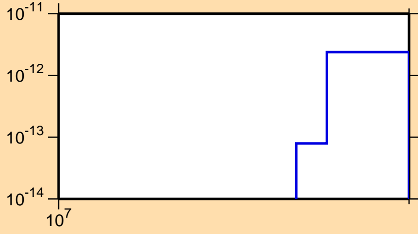
\sigma vs. E for ^{134}\text{La}(\text{mt117})
