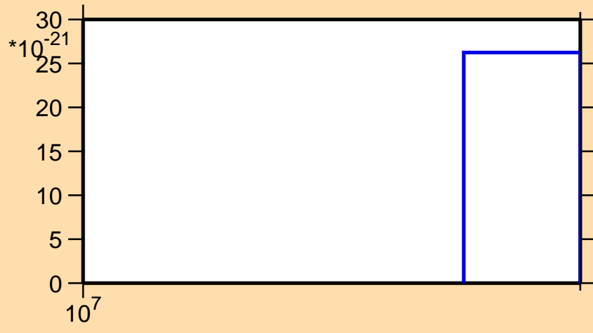
\sigma vs. E for ^{134}\text{La} (mt 11)
