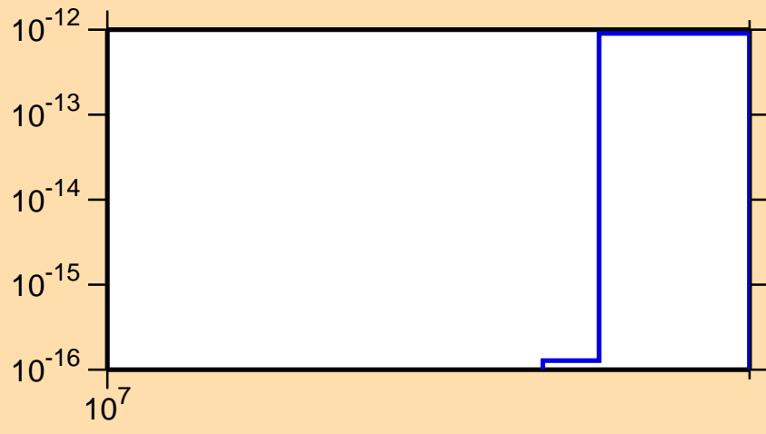
\sigma vs. E for ^{134}\text{La}(n,\text{pt})
