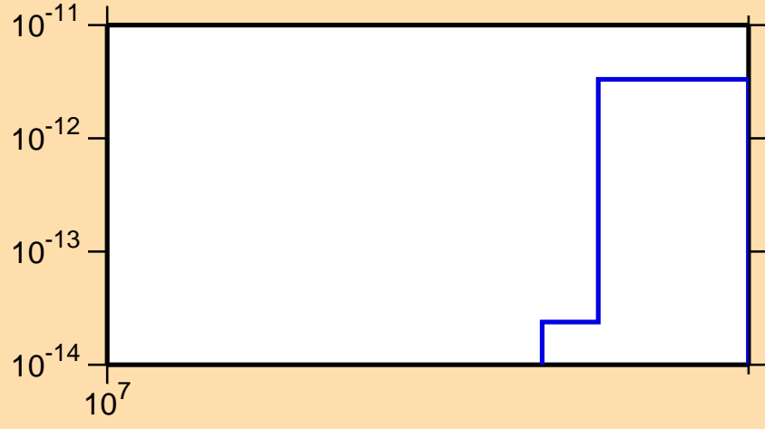
\sigma vs. E for ^{135}\text{La} (mt 45)
