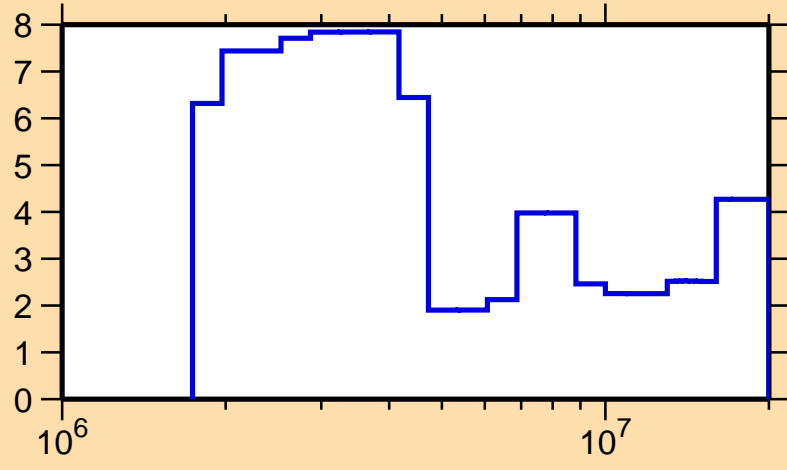
\Delta\sigma/\sigma vs. E for ^{135}\text{La}(n, el.)
