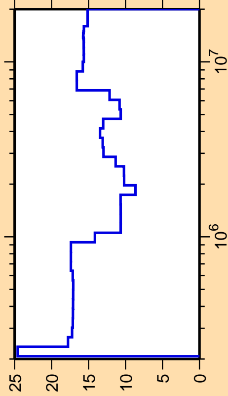
\Delta\sigma/\sigma vs. E for ^{135}\text{La}(n,n_2)
