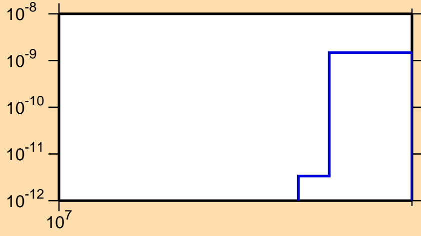
\sigma vs. E for ^{135}\text{La}(n,2n\alpha)
