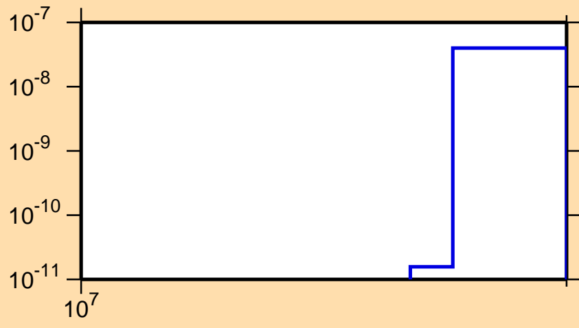
\sigma vs. E for ^{135}\text{La}(n,nt)
