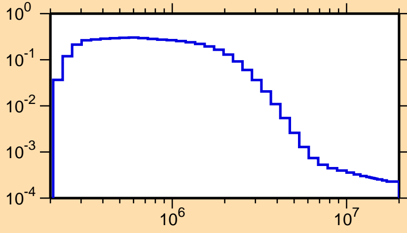
\sigma vs. E for ^{135}\text{La}(n,n_2)
