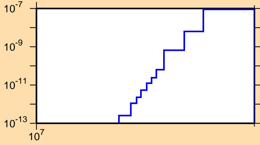
\sigma vs. E for ^{135}\text{La}(n,\text{He3})
