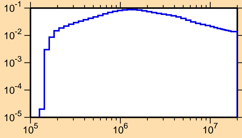
\sigma vs. E for ^{136}\text{La}(n,n_3)
