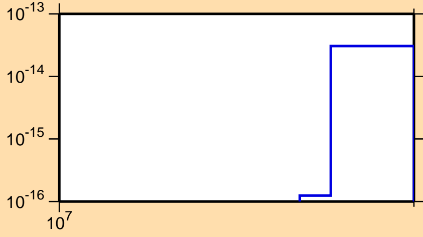
\sigma vs. E for ^{136}\text{La} (mt 34)
