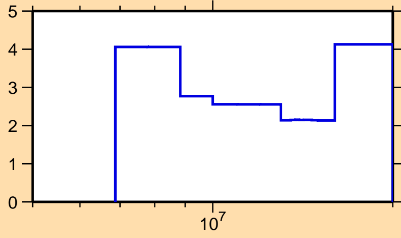
\Delta\sigma/\sigma vs. E for ^{136}\text{La}(n,\text{el.})
