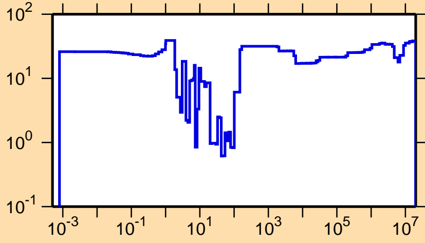
\Delta\sigma/\sigma vs. E for ^{136}\text{La}(n,\gamma)
