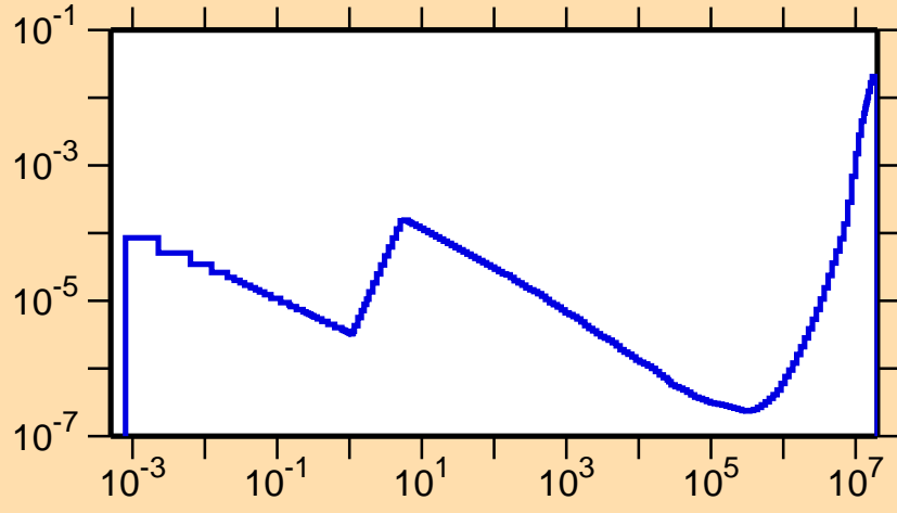
\sigma vs. E for ^{136}\text{La}(n,\alpha)
