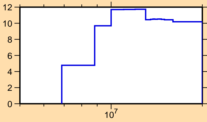
\Delta\sigma/\sigma vs. E for ^{136}\text{La}(n,\text{inel.})
