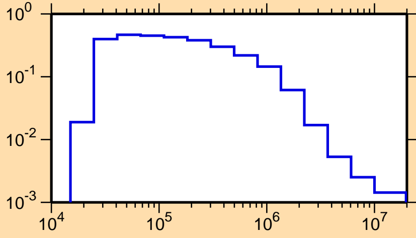
\sigma vs. E for ^{136}\text{La}(n,n_1)
