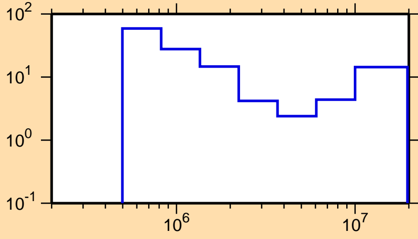
\Delta\sigma/\sigma vs. E for ^{136}\text{La}(n,n\text{cont.})
