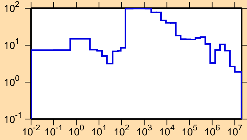
\Delta\sigma/\sigma vs. E for ^{136}\text{La}(n,el.)
