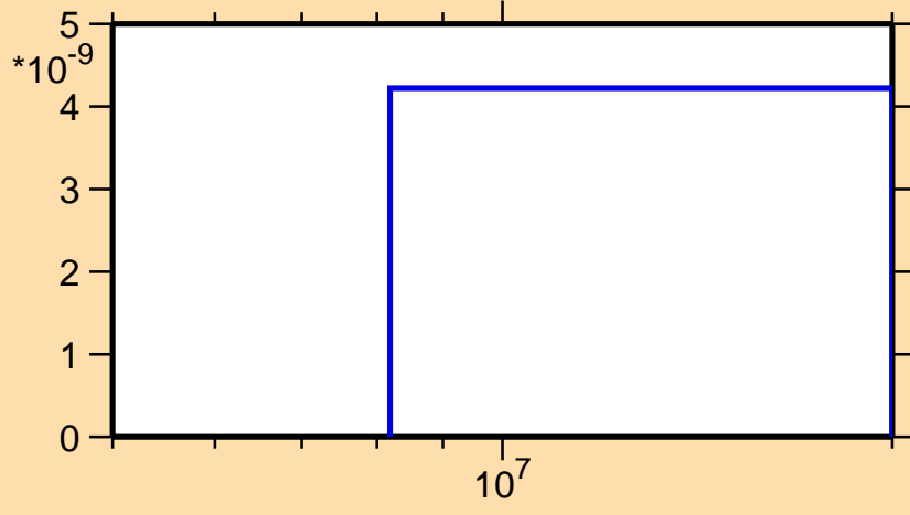
\sigma vs. E for ^{136}\text{La}(n,p\alpha)
