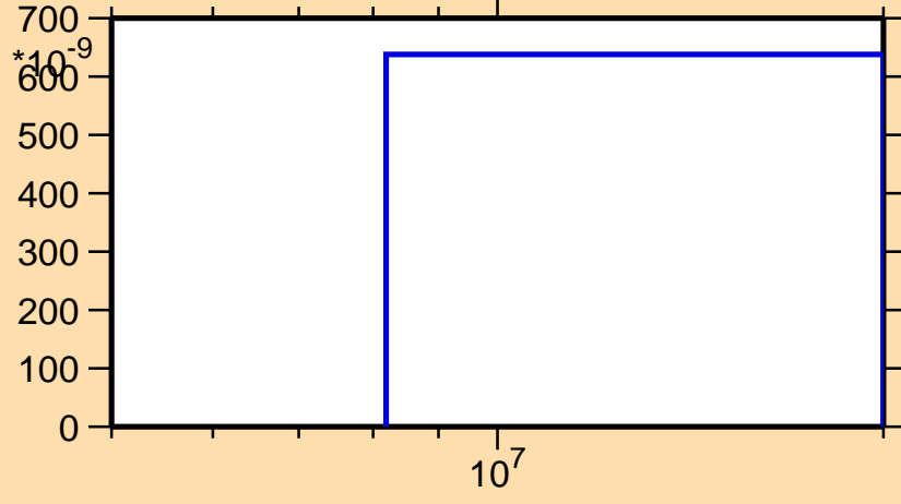
\sigma vs. E for ^{136}\text{La}(n,\text{nd})
