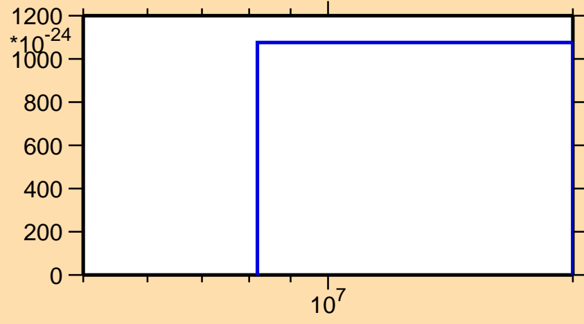
\sigma vs. E for ^{136}\text{La} (mt 11)
