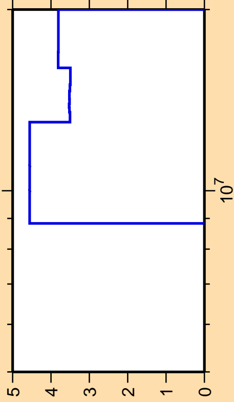
\Delta\sigma/\sigma vs. E for ^{139}\text{La}(n,2n)
