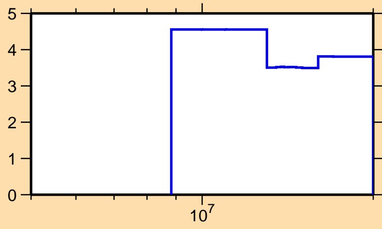
\Delta\sigma/\sigma vs. E for ^{139}\text{La}(n,2n)
