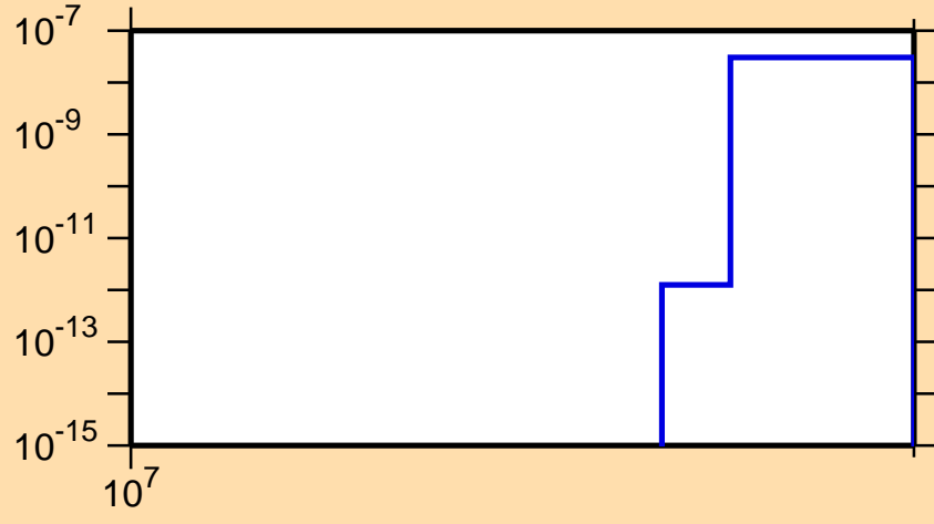
\sigma vs. E for ^{139}\text{La}(n,2np)
