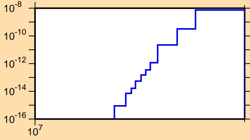
\sigma vs. E for ^{139}\text{La}(n,\text{He3})
