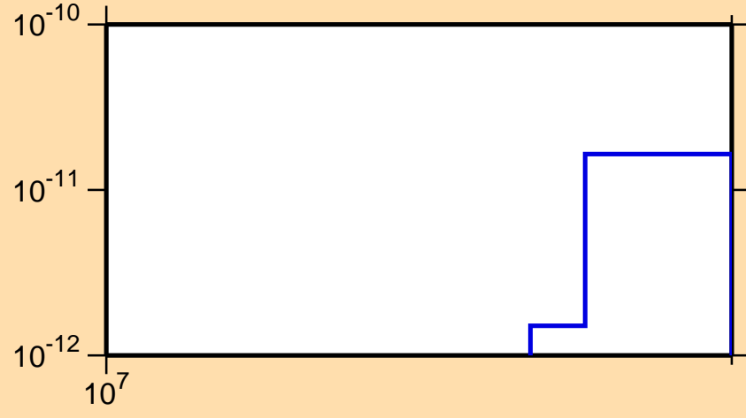
\sigma vs. E for ^{139}\text{La}(n,p\alpha)
