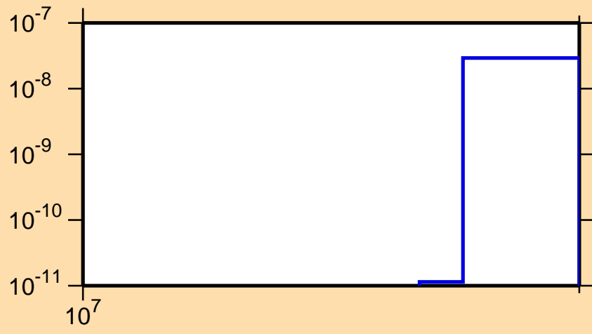
\sigma vs. E for ^{139}\text{La}(n,nt)
