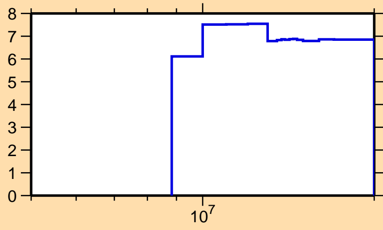
\Delta\sigma/\sigma vs. E for ^{139}\text{La}(n,\text{inel.})
