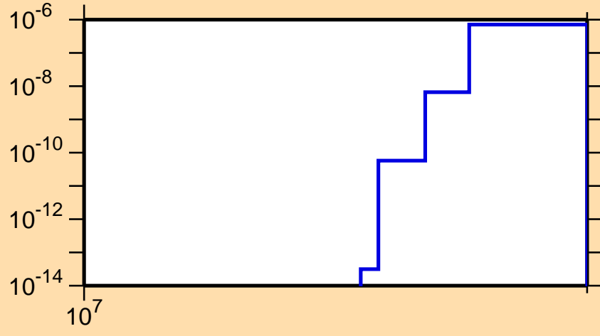
\sigma vs. E for ^{139}\text{La}(n,\text{nd})
