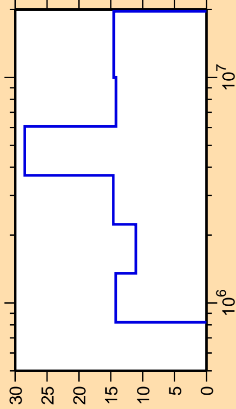
\Delta\sigma/\sigma vs. E for ^{139}\text{La}(n,n_3)
