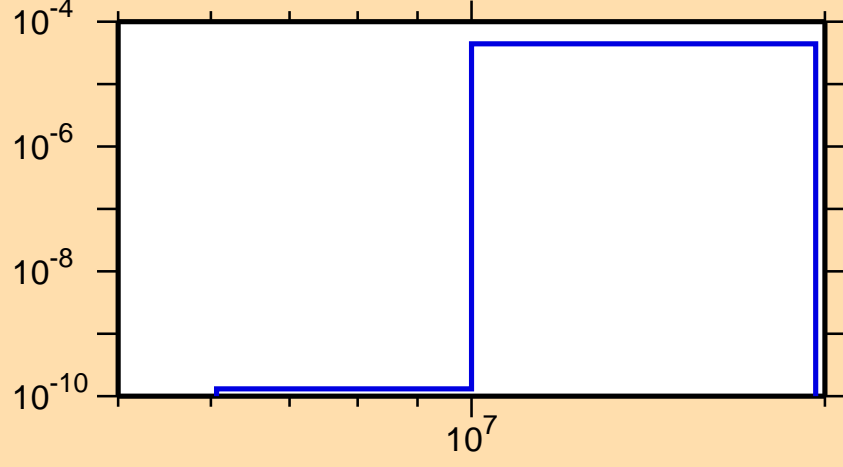
\sigma vs. E for ^{139}\text{La}(n,n\alpha)
