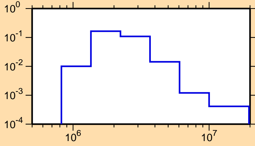
\sigma vs. E for ^{139}\text{La}(n,n_3)
