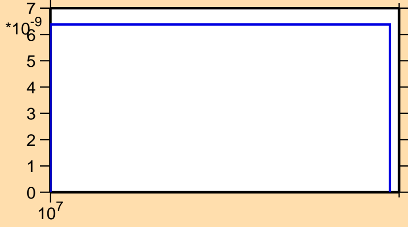
\sigma vs. E for ^{139}\text{La}(n,\text{nd})
