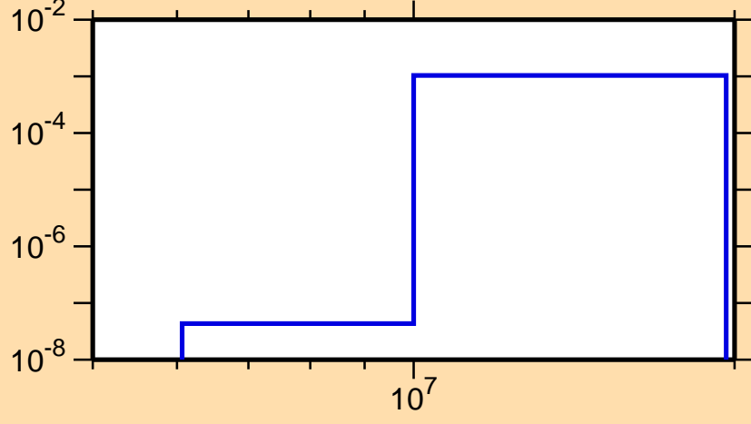
\sigma vs. E for ^{139}\text{La}(n,d)
