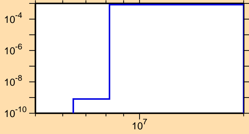
\sigma vs. E for ^{139}\text{La}(n,d)
