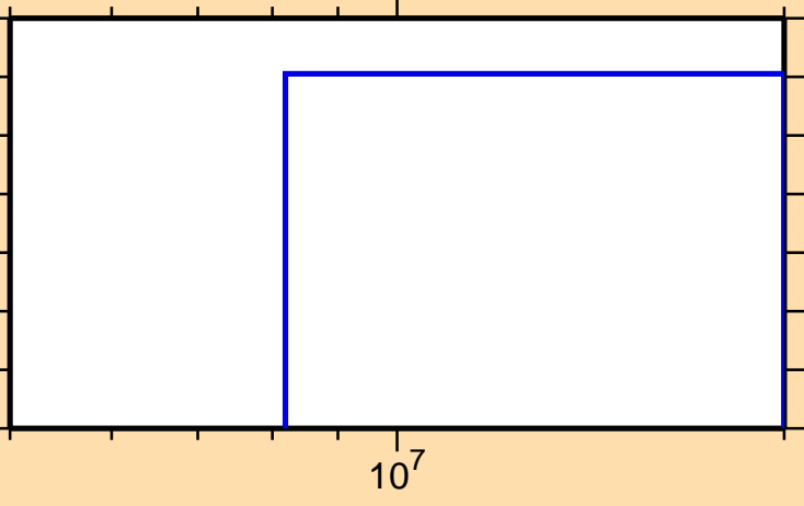
\sigma vs. E for ^{139}\text{La}(n,\text{nd})
