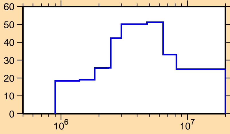
\Delta\sigma/\sigma vs. E for ^{139}\text{La}(n,\gamma)
