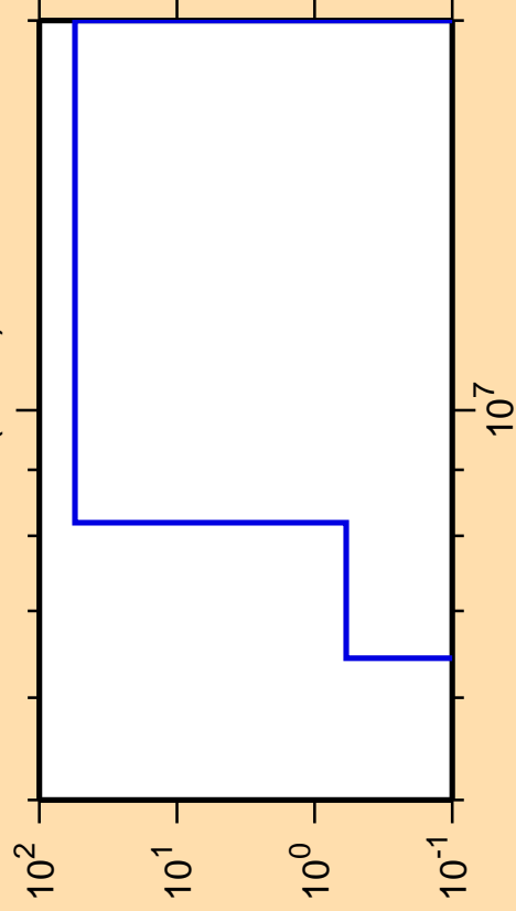
\Delta\sigma/\sigma vs. E for ^{139}\text{La}(n,n\alpha)
