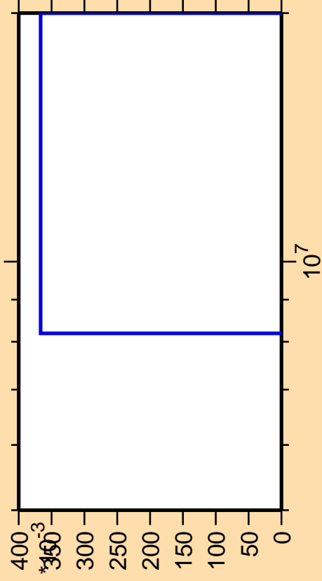
\Delta\sigma/\sigma vs. E for ^{139}\text{La}(n,p\alpha)
