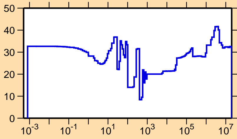
\Delta\sigma/\sigma vs. E for ^{140}\text{La}(n,\gamma)
