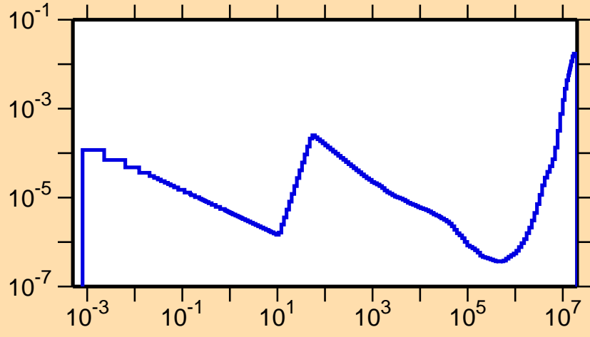
\sigma vs. E for ^{140}\text{La}(n,\alpha)
