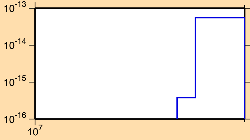
\sigma vs. E for ^{140}\text{La} (mt 34)
