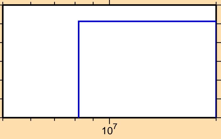
\sigma vs. E for ^{140}\text{La}(n,\text{nd})
