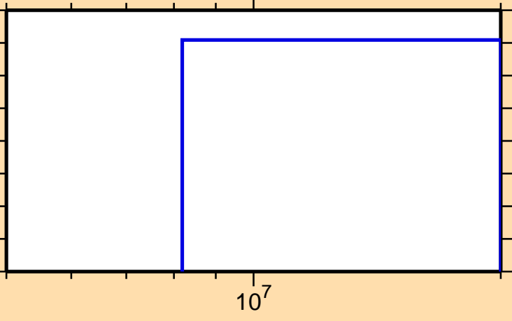
\sigma vs. E for ^{140}\text{La}(n,\text{He3})
