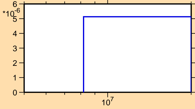
\sigma vs. E for ^{140}\text{La}(n,\text{nd})
