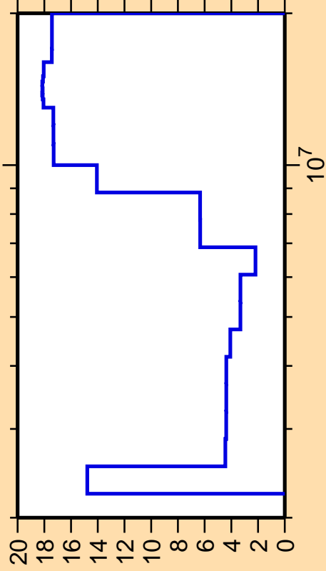
\Delta\sigma/\sigma vs. E for ^{141}\text{La}(n,\text{ncont.})
