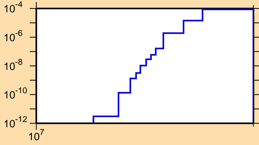
\sigma vs. E for ^{141}\text{La}(n,nt)
