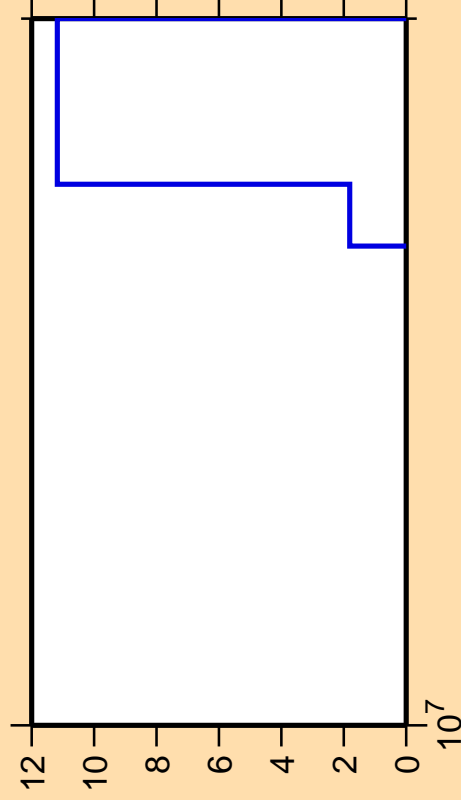
\Delta\sigma/\sigma vs. E for ^{141}\text{La} (mt117)
