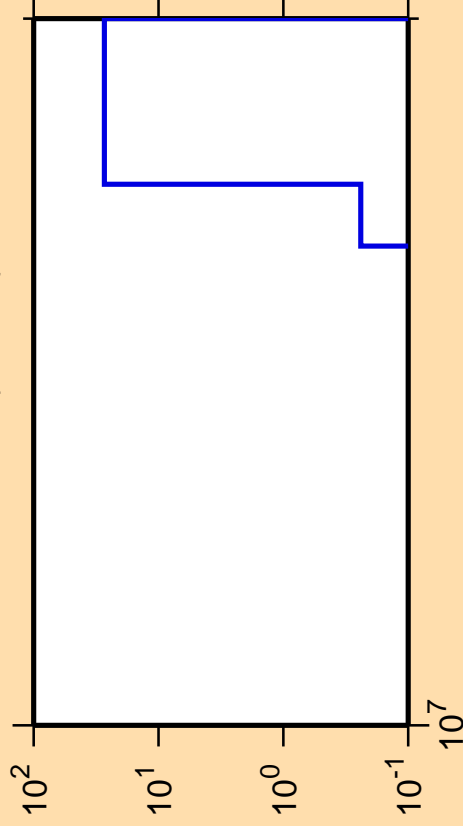
\Delta\sigma/\sigma vs. E for ^{141}\text{La}(n,\text{He3})
