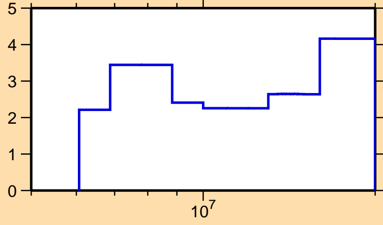
\Delta\sigma/\sigma vs. E for ^{141}\text{La}(n,\text{el.})
