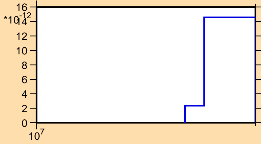
\sigma vs. E for ^{141}\text{La} (mt117)
