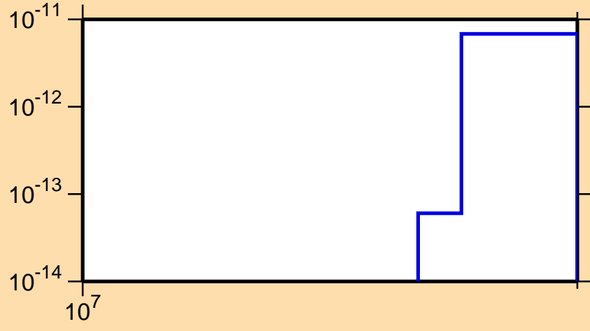
\sigma vs. E for ^{141}\text{La}(n,\text{He3})
