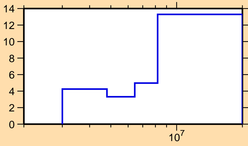
\Delta\sigma/\sigma vs. E for ^{141}\text{La}(n,n\text{cont.})
