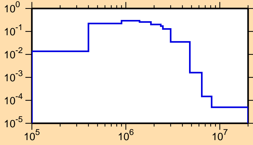
\sigma vs. E for ^{141}\text{La}(n,n_2)
