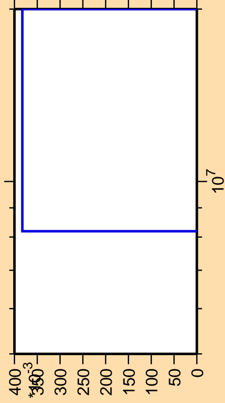
\Delta\sigma/\sigma vs. E for ^{141}\text{La}(n,p\alpha)
