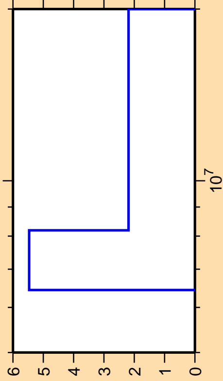
\Delta\sigma/\sigma vs. E for ^{141}\text{La}(n,2n)
