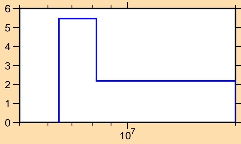
\Delta\sigma/\sigma vs. E for ^{141}\text{La}(n,2n)
