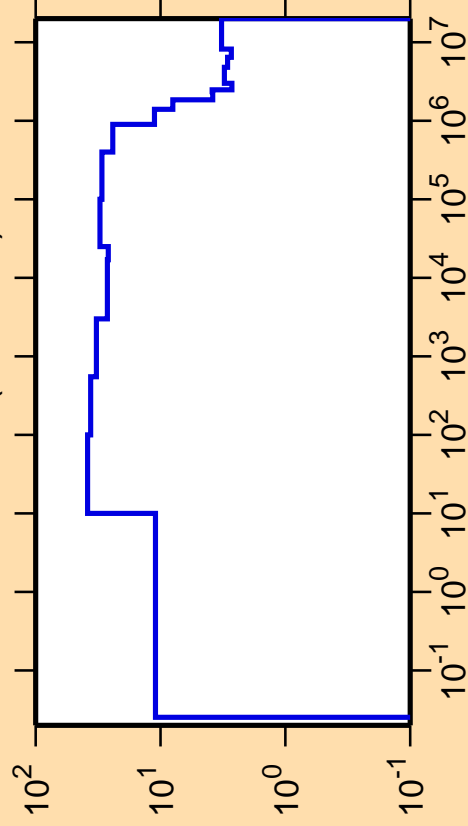
\Delta\sigma/\sigma vs. E for ^{142}\text{La}(n,\text{nonel.})
