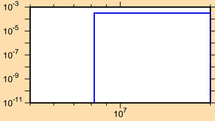
\sigma vs. E for ^{142}\text{La}(n,np)
