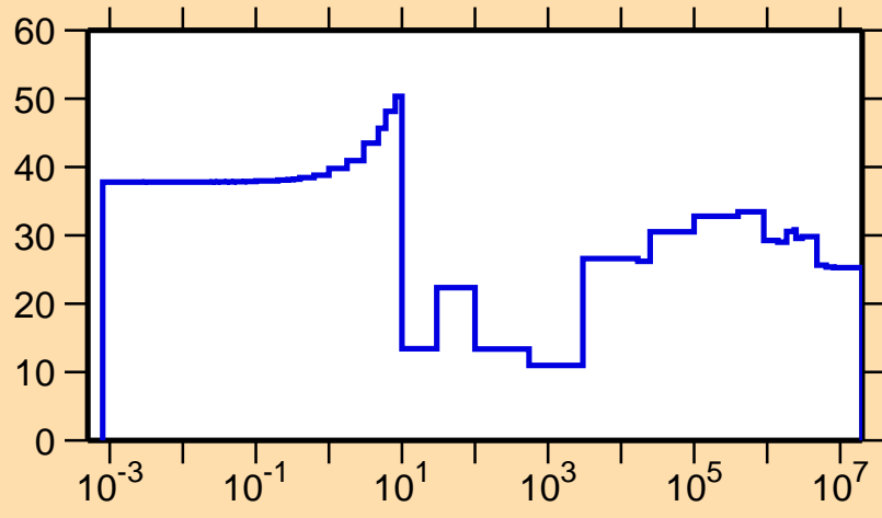
\Delta\sigma/\sigma vs. E for ^{142}\text{La}(n,\gamma)
