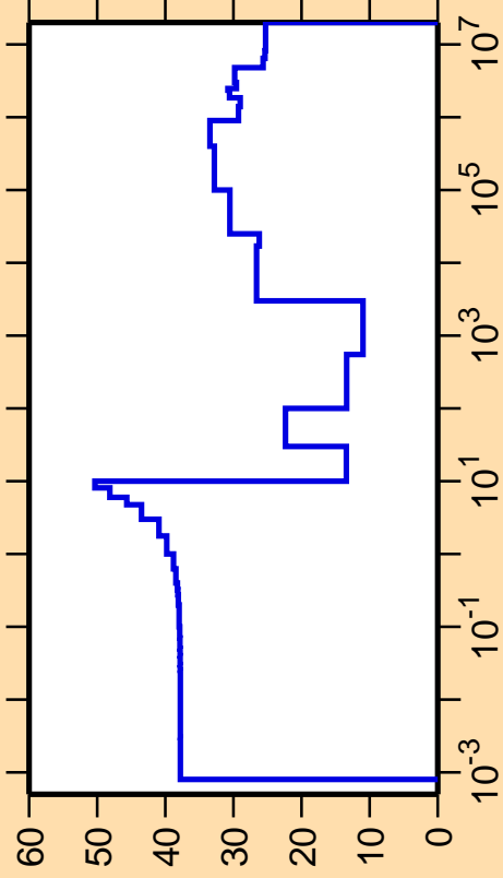
\Delta\sigma/\sigma vs. E for ^{142}\text{La}(n,\gamma)
