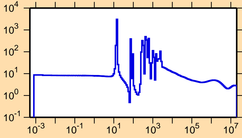
\sigma vs. E for ^{143}\text{La}(n,\text{el.})
