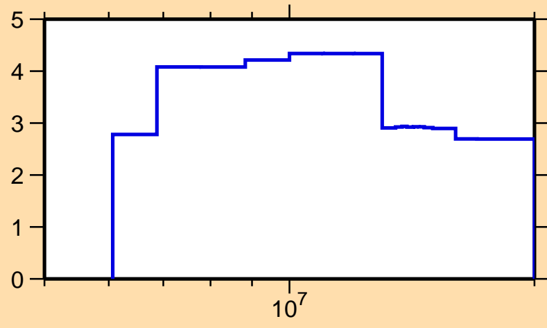
\Delta\sigma/\sigma vs. E for ^{143}\text{La}(n,\text{el.})
