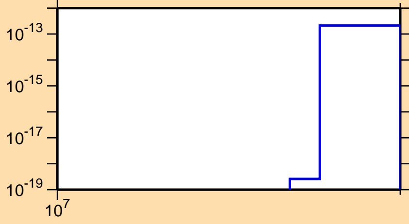
\sigma vs. E for ^{143}\text{La}(n,\text{He3})
