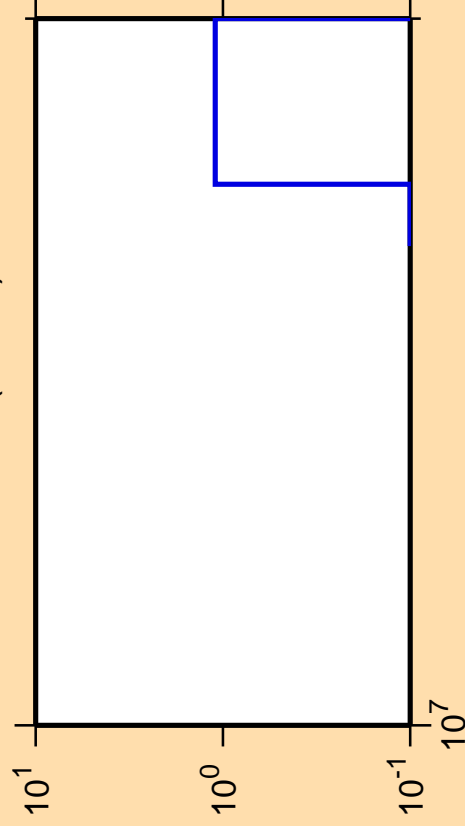
\Delta\sigma/\sigma vs. E for ^{143}\text{La} (mt 11)
