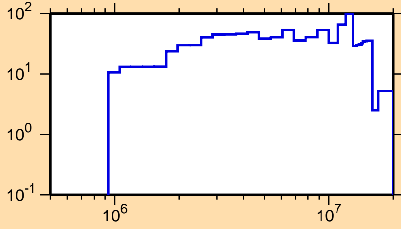
\Delta\sigma/\sigma vs. E for ^{143}\text{La}(n,n_1)
