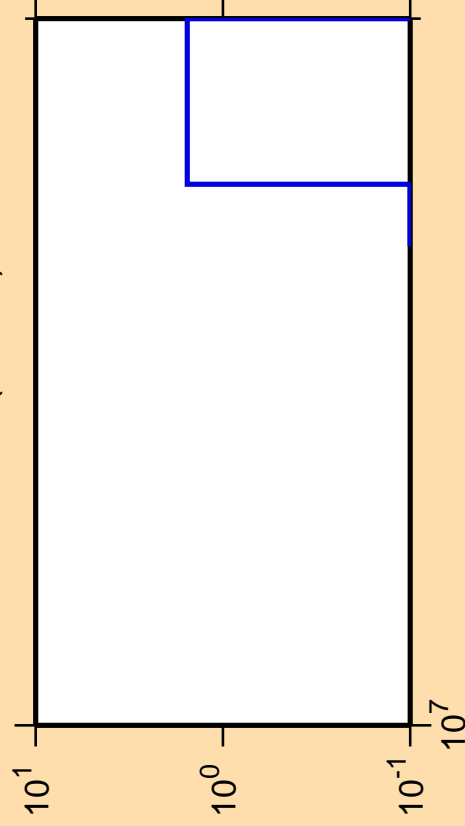
\Delta\sigma/\sigma vs. E for ^{143}\text{La}(n,\text{He3})
