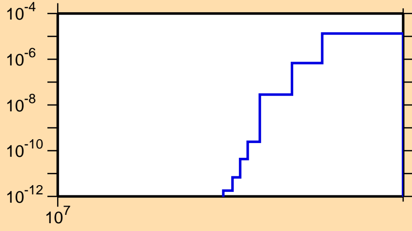
\sigma vs. E for ^{143}\text{La}(n,\text{nd})
