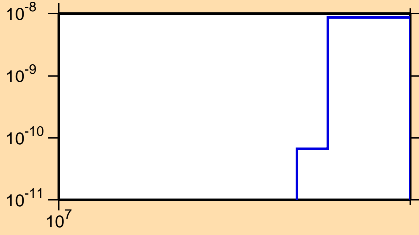
\sigma vs. E for ^{143}\text{La}(n,3n\alpha)
