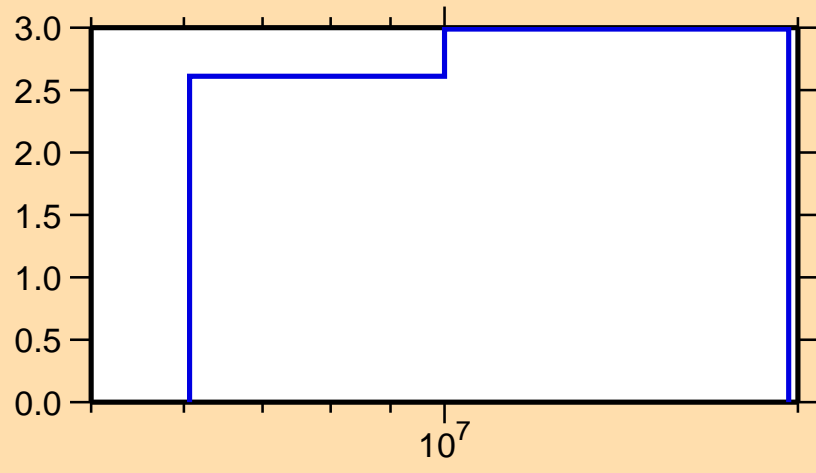
\Delta\sigma/\sigma vs. E for ^{143}\text{La}(n,\text{el.})
