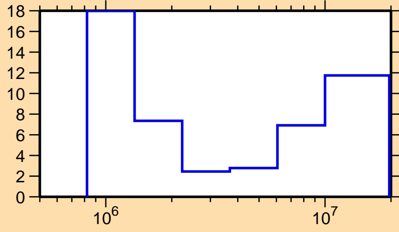
\Delta\sigma/\sigma vs. E for ^{143}\text{La}(n,\text{inel.})
