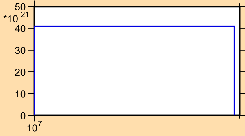
\sigma vs. E for ^{143}\text{La} (mt 42)
