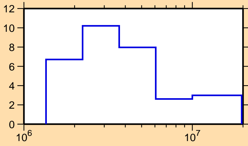
\Delta\sigma/\sigma vs. E for ^{143}\text{La}(n,\text{el.})
