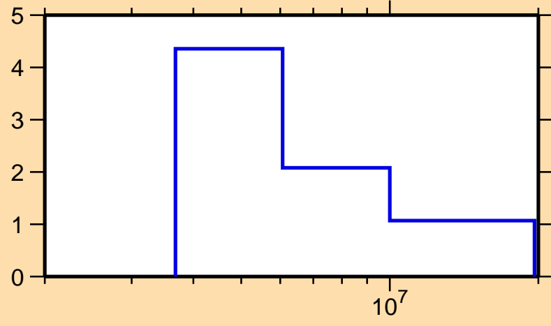
\Delta\sigma/\sigma vs. E for ^{143}\text{La}(n,\text{tot.})
