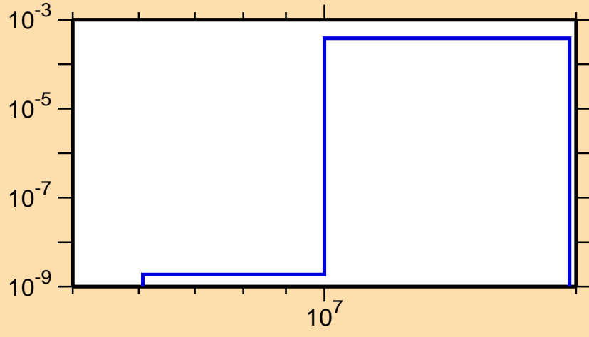
\sigma vs. E for ^{143}\text{La}(n,d)
