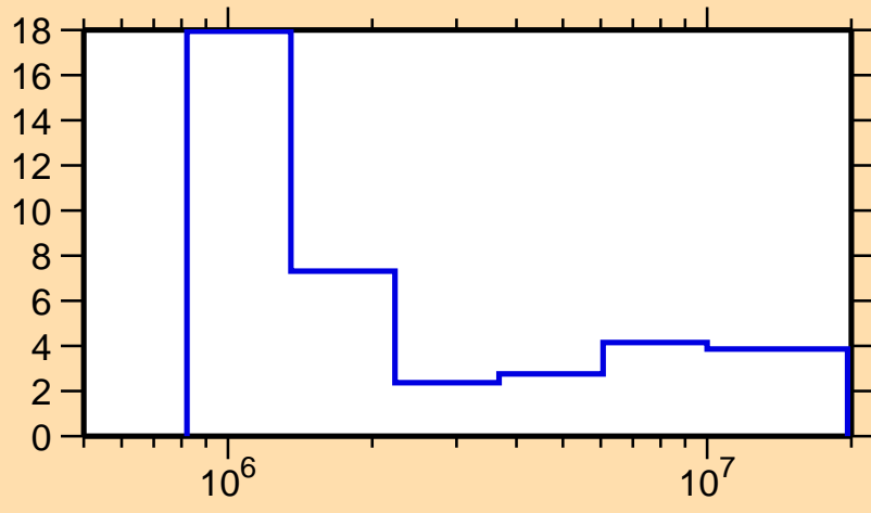
\Delta\sigma/\sigma vs. E for ^{143}\text{La}(n,\text{nonel.})
