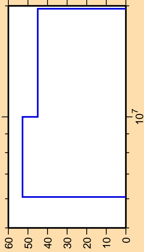
\Delta\sigma/\sigma vs. E for ^{143}\text{La}(n,p)
