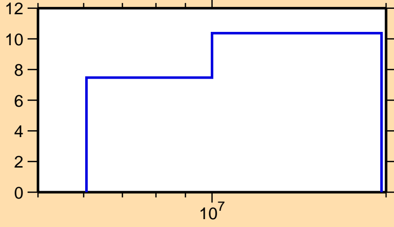
\Delta\sigma/\sigma vs. E for ^{143}\text{La}(n,2n)
