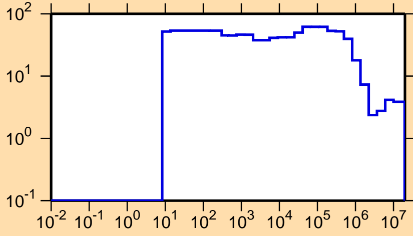
\Delta\sigma/\sigma vs. E for ^{143}\text{La}(n,\text{nonel.})
