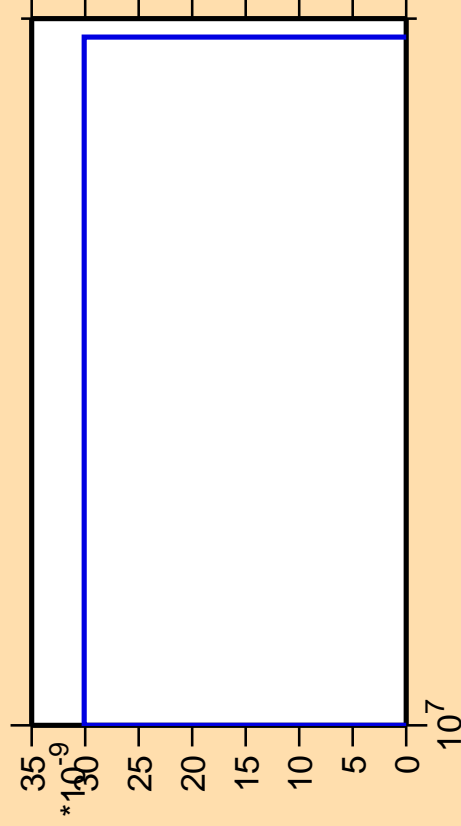
\Delta\sigma/\sigma vs. E for ^{143}\text{La} (mt 42)
