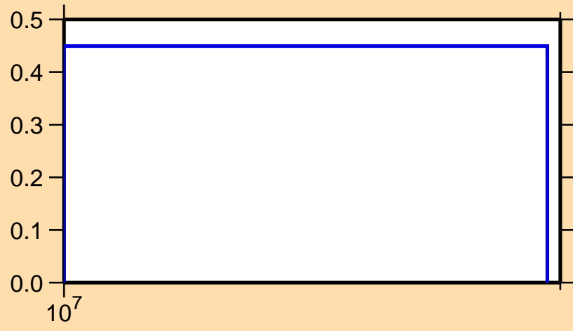
\sigma vs. E for ^{143}\text{La}(n,3n)
