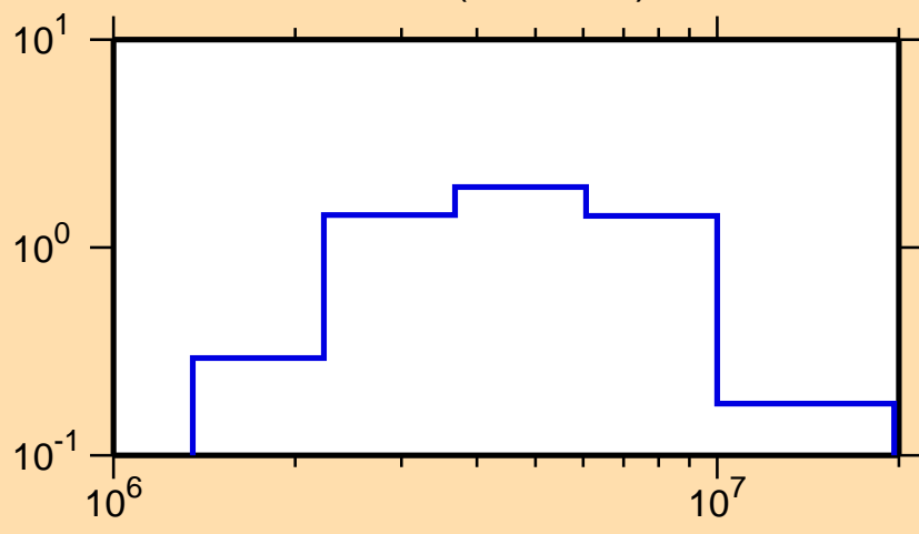
\sigma vs. E for ^{143}\text{La}(n,n\text{cont.})
