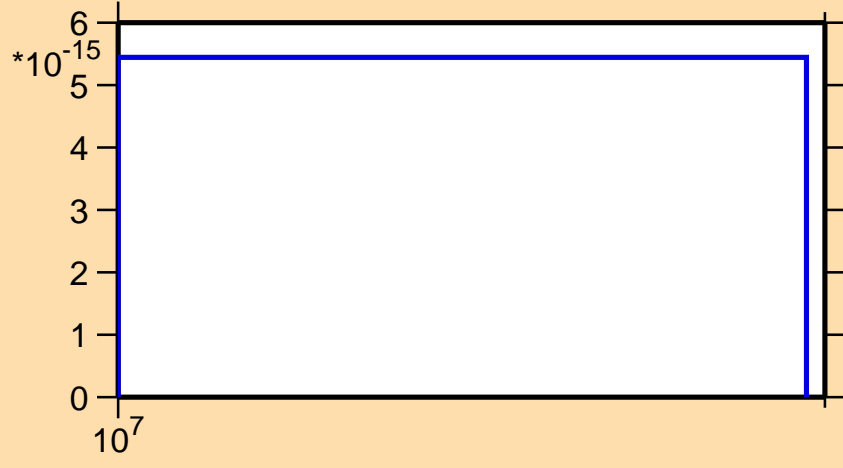
\sigma vs. E for ^{143}\text{La} (mt 11)
