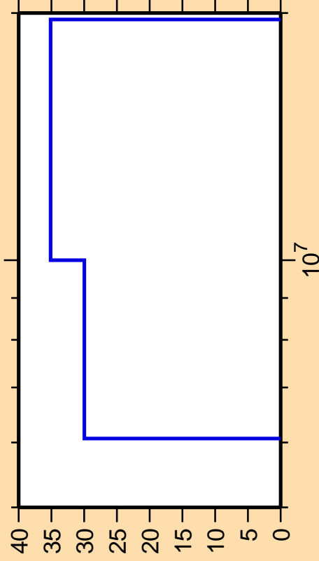
\Delta\sigma/\sigma vs. E for ^{143}\text{La}(n,\gamma)
