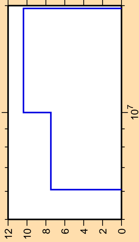
\Delta\sigma/\sigma vs. E for ^{143}\text{La}(n,2n)
