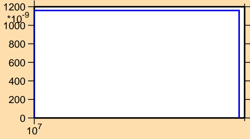
\sigma vs. E for ^{143}\text{La}(n,nt)
