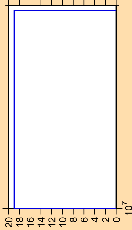
\Delta\sigma/\sigma vs. E for ^{143}\text{La}(n,3n)
