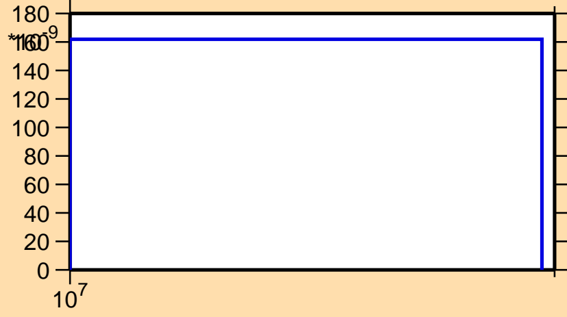
\sigma vs. E for ^{143}\text{La}(n,\text{nd})
