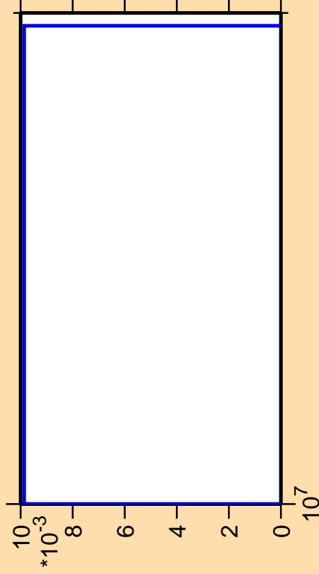
\Delta\sigma/\sigma vs. E for ^{143}\text{La}(n,\text{He3})
