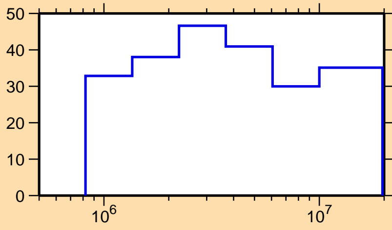
\Delta\sigma/\sigma vs. E for ^{143}\text{La}(n,\gamma)
