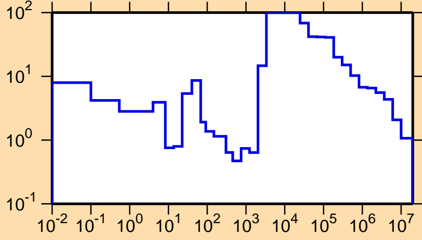
\Delta\sigma/\sigma vs. E for ^{143}\text{La}(n,\text{tot.})
