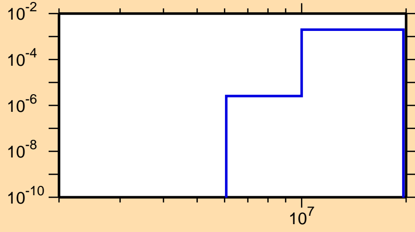
\sigma vs. E for ^{143}\text{La}(n,p)
