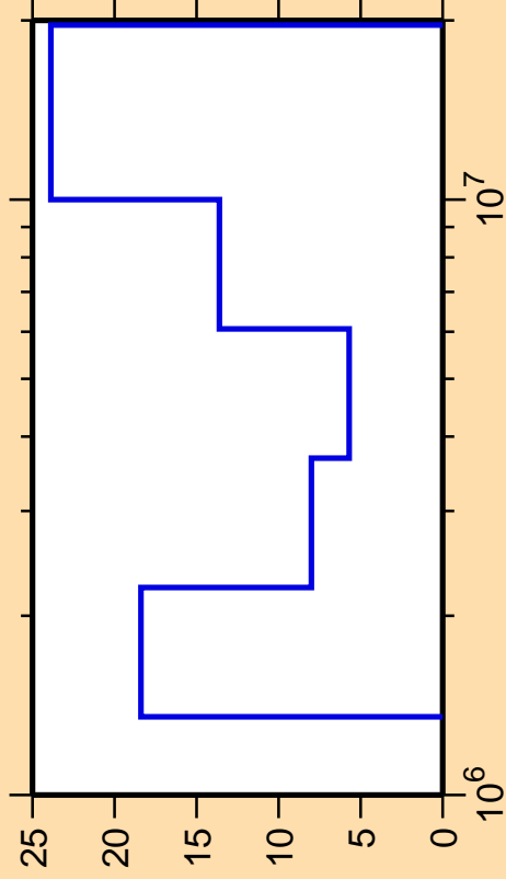
\Delta\sigma/\sigma vs. E for ^{143}\text{La}(n,n\text{cont.})
