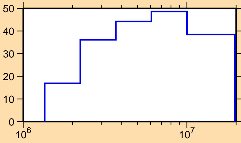
\Delta\sigma/\sigma vs. E for ^{143}\text{La}(n,n_1)
