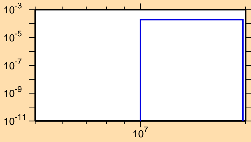
\sigma vs. E for ^{143}\text{La}(n,np)
