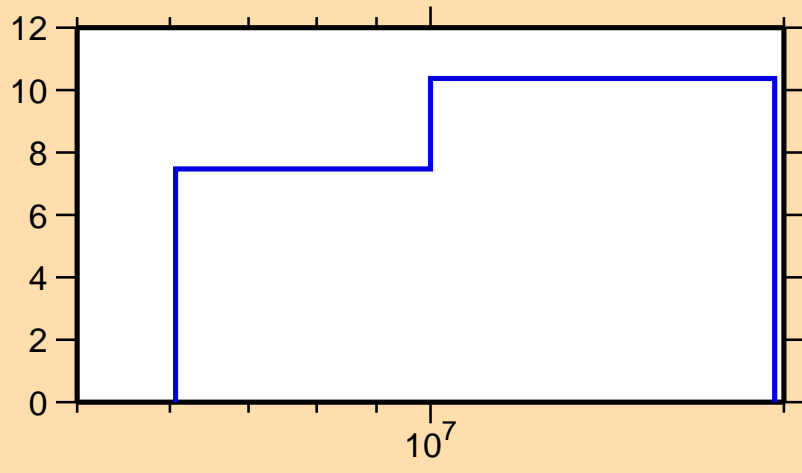
\Delta\sigma/\sigma vs. E for ^{143}\text{La}(n,2n)
