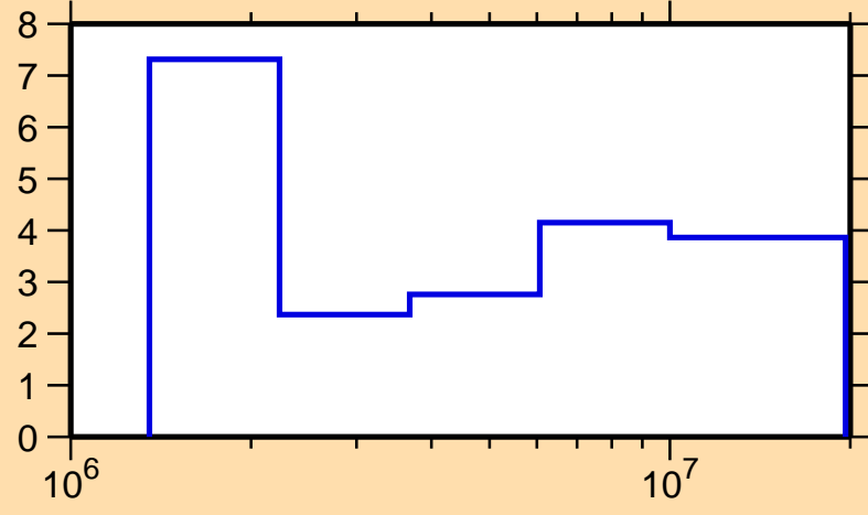
\Delta\sigma/\sigma vs. E for ^{143}\text{La}(n,\text{nonel.})
