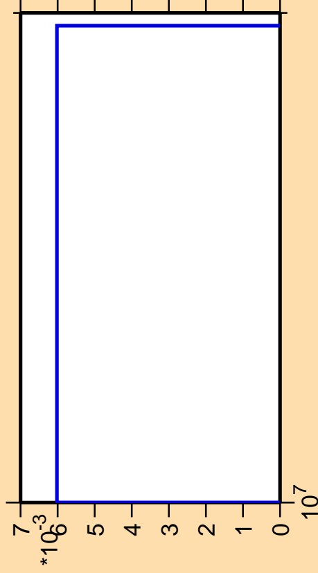
\Delta\sigma/\sigma vs. E for ^{143}\text{La} (mt 11)
