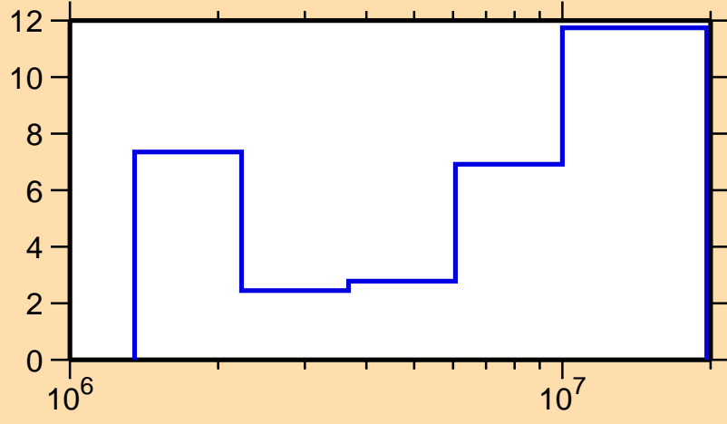
\Delta\sigma/\sigma vs. E for ^{143}\text{La}(n,\text{inel.})
