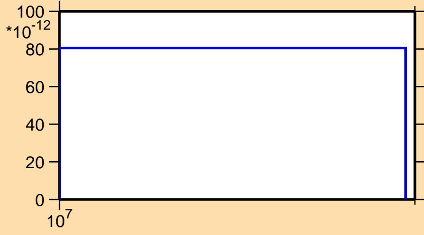
\sigma vs. E for ^{143}\text{La}(n,3n\alpha)
