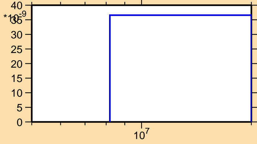
\sigma vs. E for ^{143}\text{La}(n,2n\alpha)
