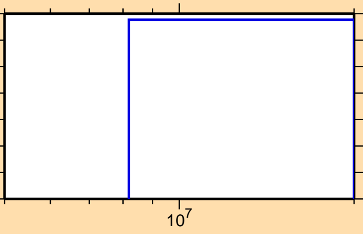
\sigma vs. E for ^{143}\text{La}(n,2np)
