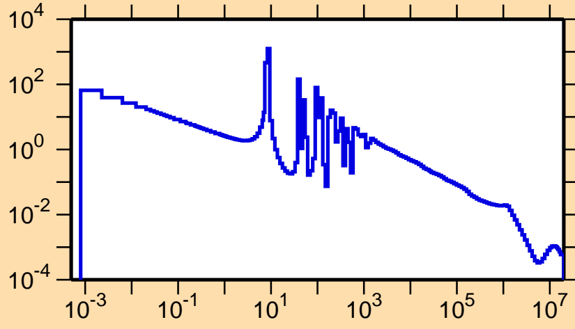
\sigma vs. E for ^{144}\text{La}(n,\gamma)
