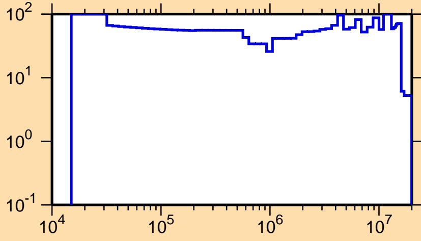
\Delta\sigma/\sigma vs. E for ^{144}\text{La}(n,n_1)
