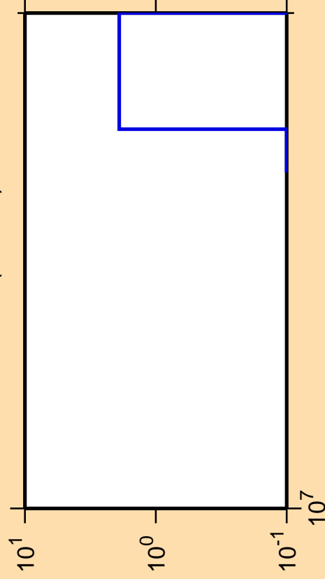
\Delta\sigma/\sigma vs. E for ^{144}\text{La}(n,\text{He}3)
