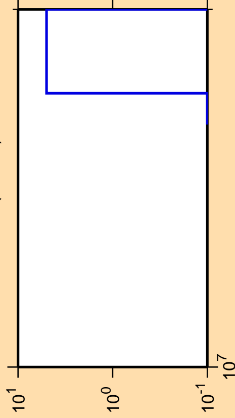
\Delta\sigma/\sigma vs. E for ^{144}\text{La} (mt 11)
