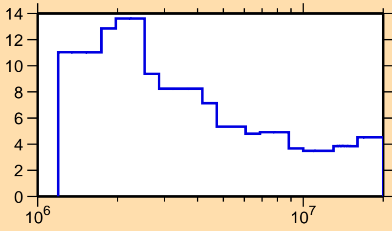
\Delta\sigma/\sigma vs. E for ^{144}\text{La}(n,\text{tot.})
