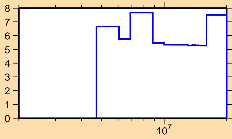
\Delta\sigma/\sigma vs. E for ^{144}\text{La}(n,\text{el.})
