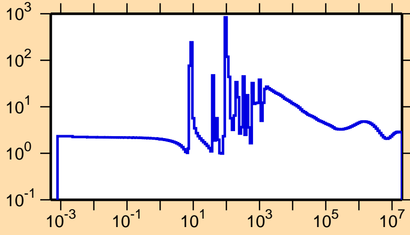
\sigma vs. E for ^{144}\text{La}(n,\text{el.})
