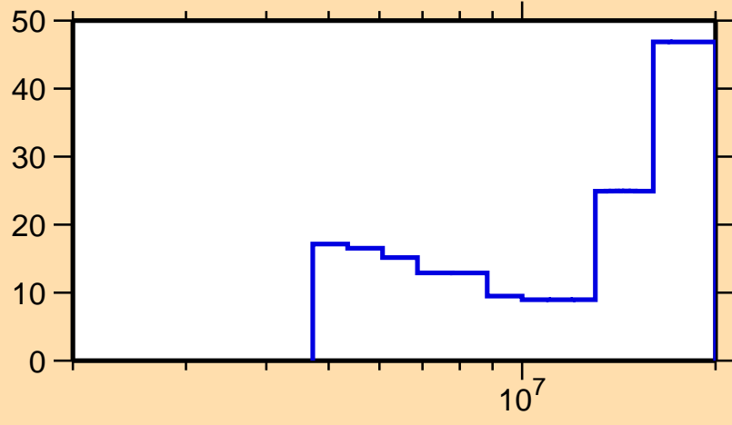
\Delta\sigma/\sigma vs. E for ^{144}\text{La}(n,2n)
