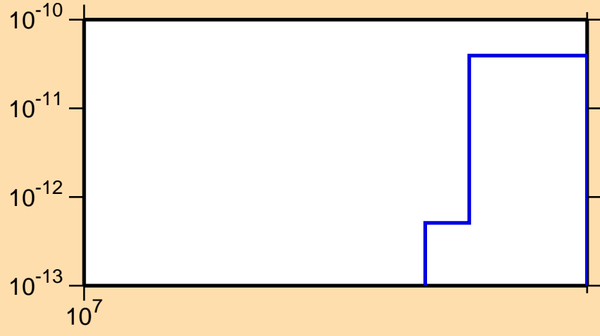
\sigma vs. E for ^{144}\text{La}(n,3n\alpha)
