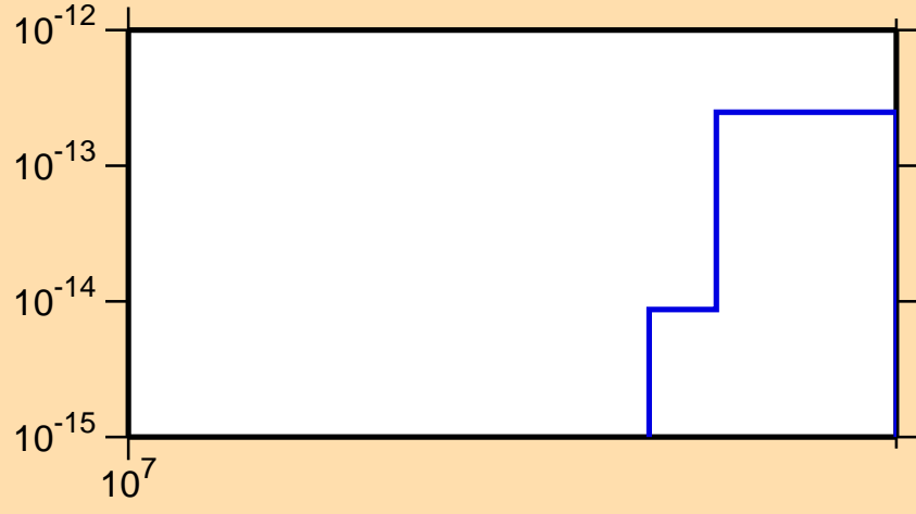
\sigma vs. E for ^{144}\text{La}(n,\text{He}3)
