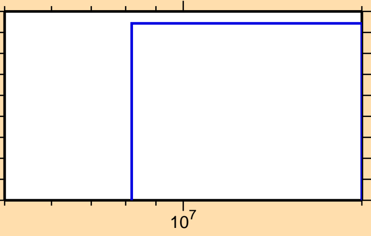
\sigma vs. E for ^{144}\text{La}(n,nt)
