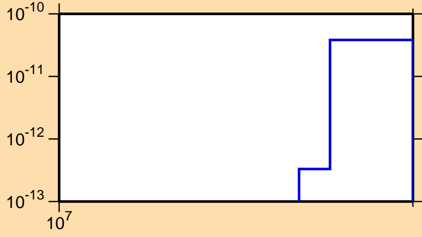
\sigma vs. E for ^{145}\text{La}(n,3n\alpha)
