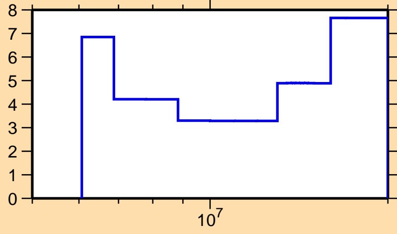
\Delta\sigma/\sigma vs. E for ^{145}\text{La}(n,\text{tot.})
