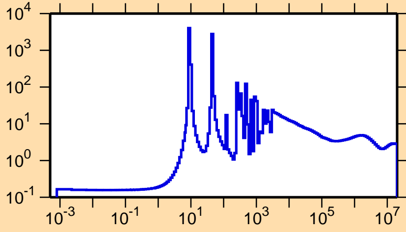
\sigma vs. E for ^{145}\text{La}(n,\text{el.})
