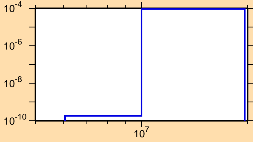
\sigma vs. E for ^{145}\text{La}(n,n\alpha)
