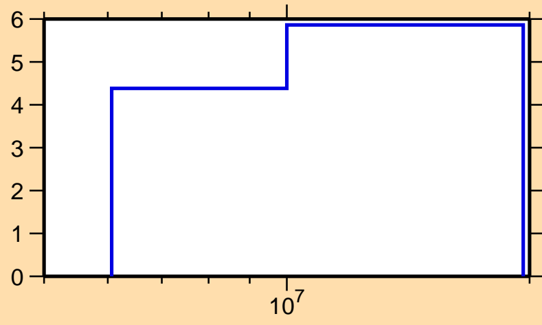
\Delta\sigma/\sigma vs. E for ^{145}\text{La}(n,\text{el.})
