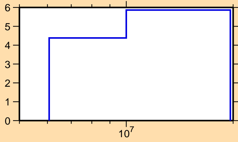
\Delta\sigma/\sigma vs. E for ^{145}\text{La}(n,el.)
