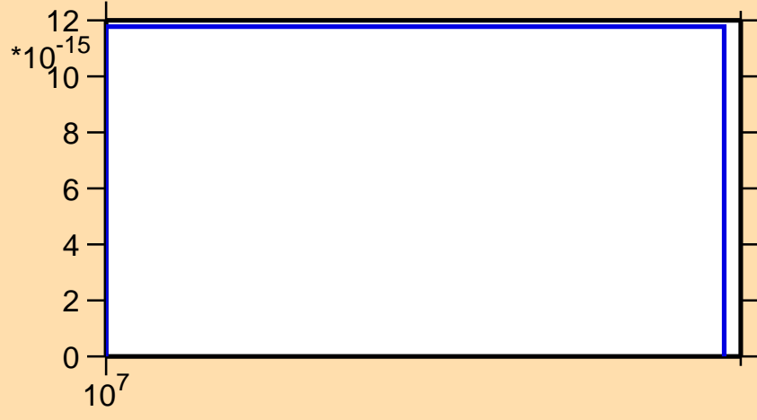
\sigma vs. E for ^{146}\text{La}(n,3n\alpha)
