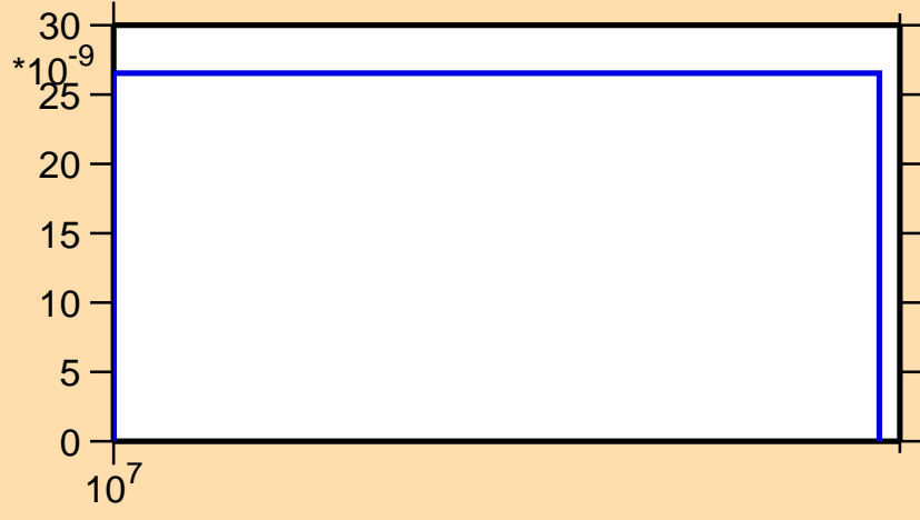
\sigma vs. E for ^{146}\text{La}(n,2np)
