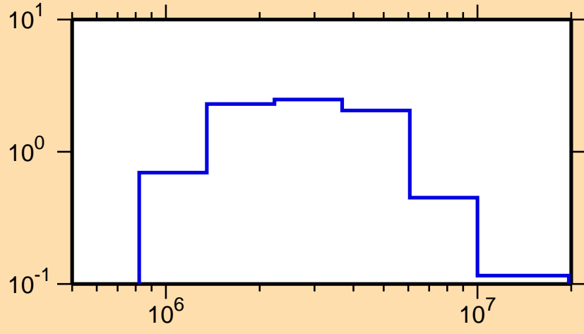
\sigma vs. E for ^{146}\text{La}(n,n\text{cont.})
