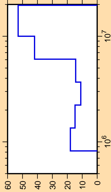
\Delta\sigma/\sigma vs. E for ^{146}\text{La}(n,n\text{cont.})
