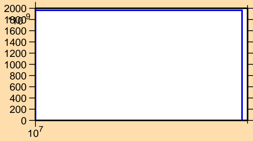
\sigma vs. E for ^{146}\text{La}(n,nt)
