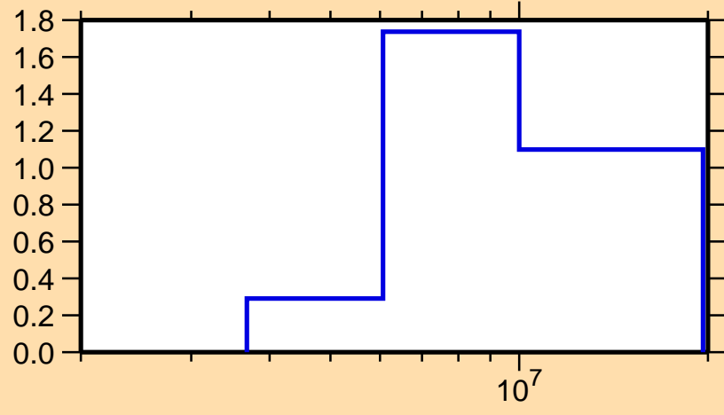
\sigma vs. E for ^{146}\text{La}(n,2n)
