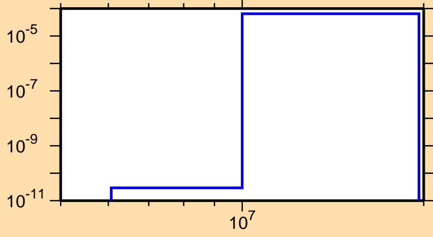
\sigma vs. E for ^{146}\text{La}(n,n\alpha)
