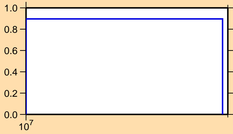
\sigma vs. E for ^{146}\text{La}(n,3n)
