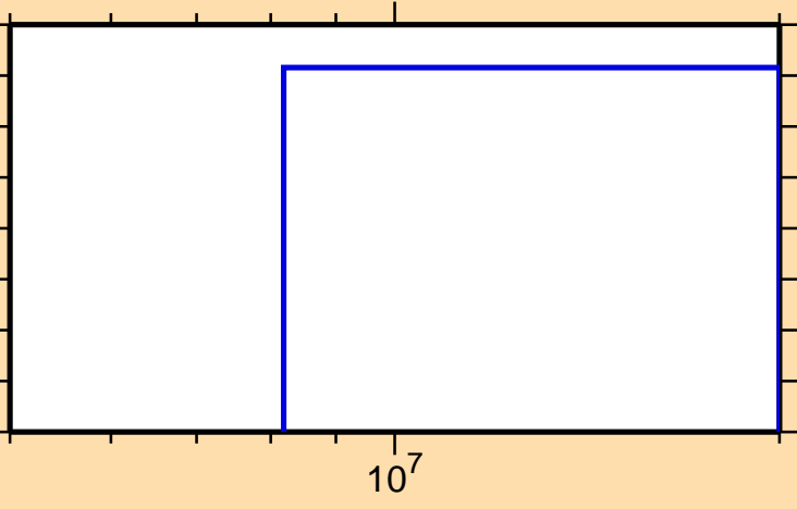
\sigma vs. E for ^{146}\text{La}(n,d)
