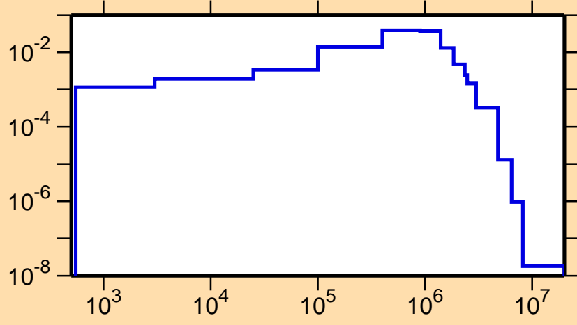
\sigma vs. E for ^{146}\text{La}(n,n_1)
