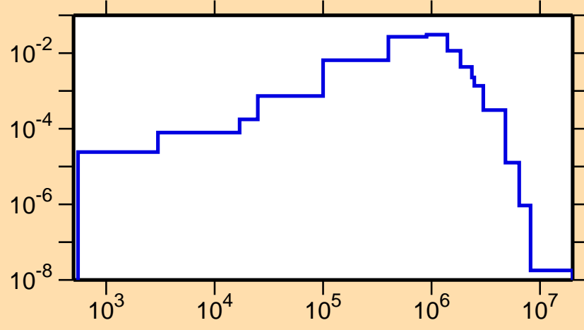
\sigma vs. E for ^{146}\text{La}(n,n_3)
