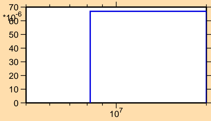
\sigma vs. E for ^{146}\text{La}(n,np)
