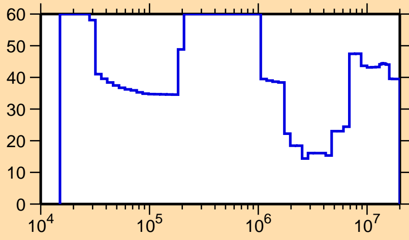
\Delta\sigma/\sigma vs. E for ^{147}\text{La}(n,\text{inel.})
