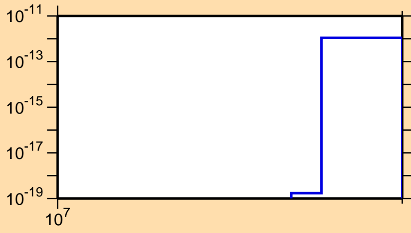
\sigma vs. E for ^{147}\text{La} (mt 11)
