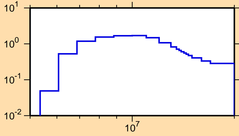
\sigma vs. E for ^{147}\text{La}(n,2n)
