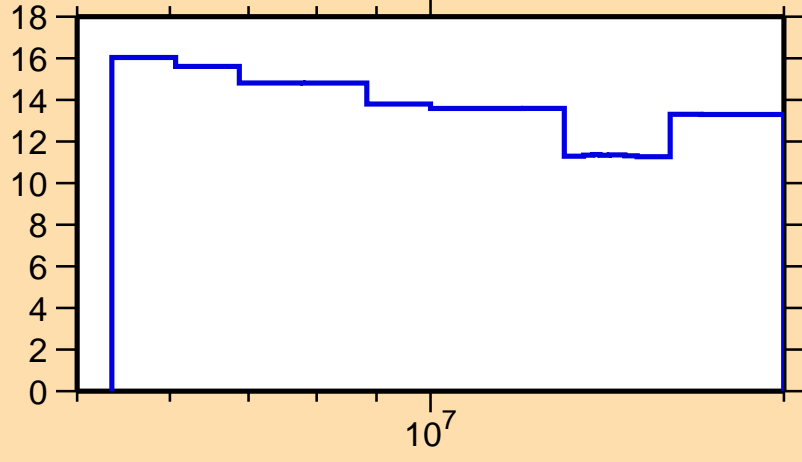
\Delta\sigma/\sigma vs. E for ^{147}\text{La}(n,\text{nonel.})
