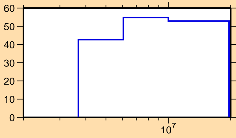
\Delta\sigma/\sigma vs. E for ^{147}\text{La}(n,n\text{cont.})
