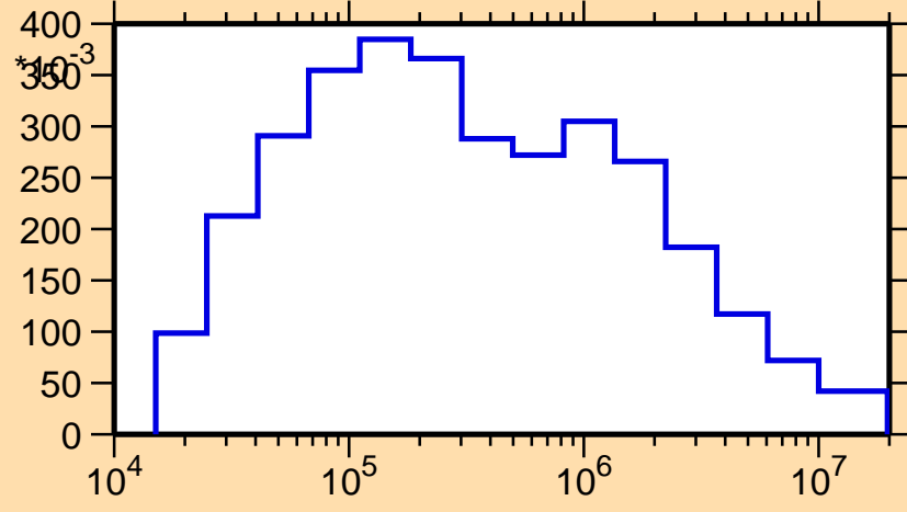
\sigma vs. E for ^{147}\text{La}(n,n_1)
