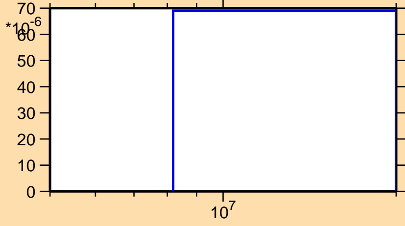
\sigma vs. E for ^{147}\text{La}(n,d)
