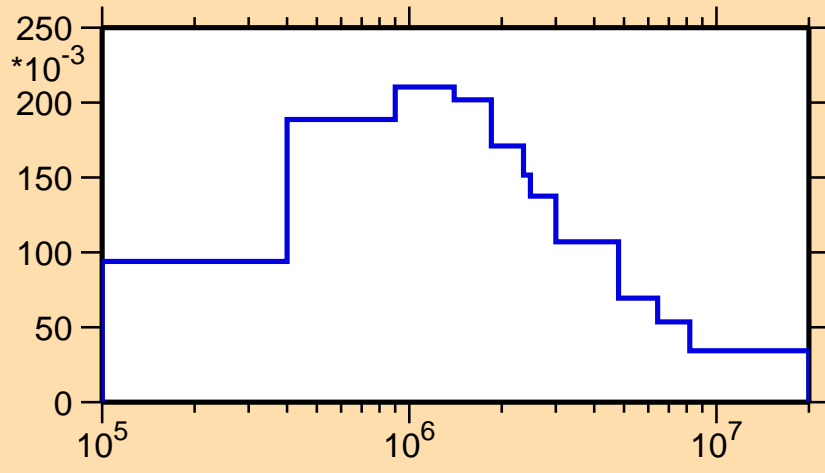
\sigma vs. E for ^{147}\text{La}(n,n_4)
