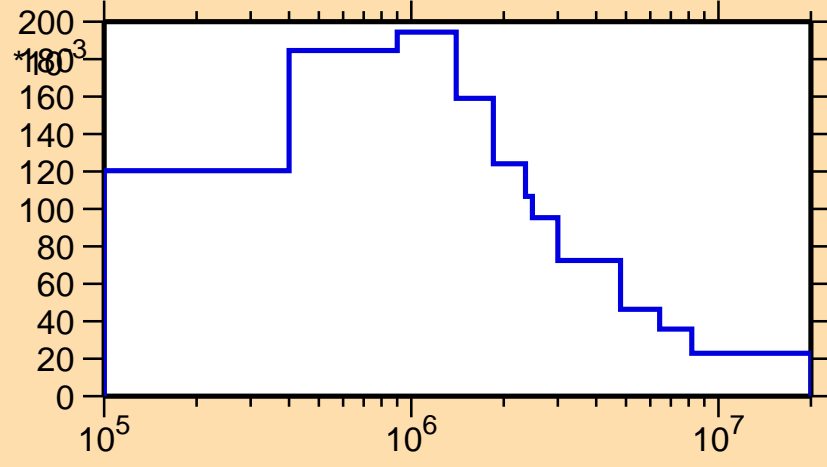
\sigma vs. E for ^{147}\text{La}(n,n_3)
