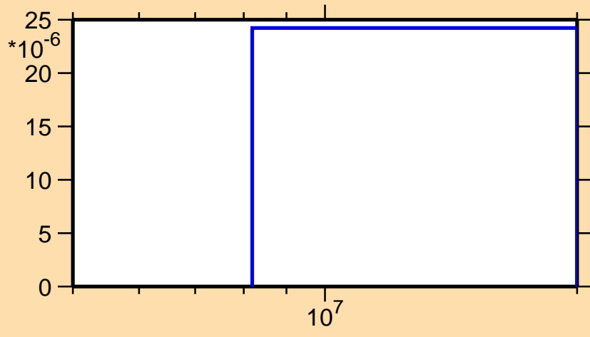
\sigma vs. E for ^{147}\text{La}(n,np)
