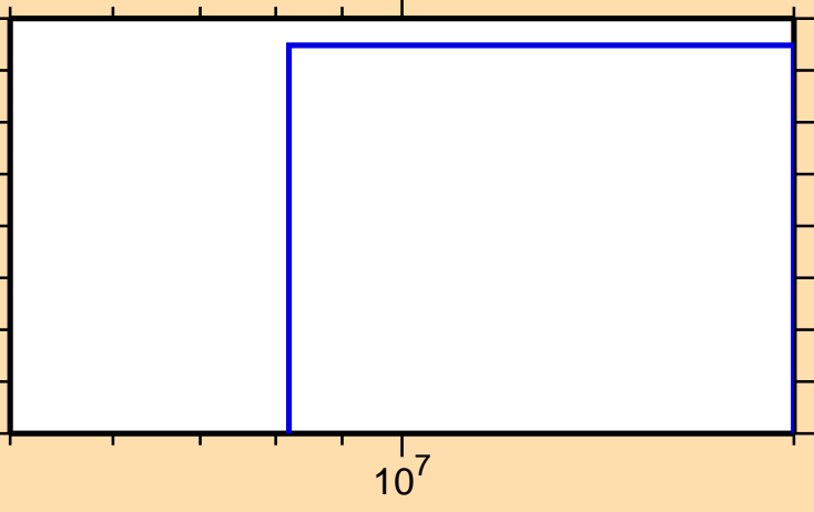
\sigma vs. E for ^{147}\text{La} (mt 42)
